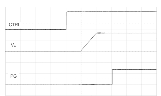
Start-up enabled by CTRL signal. T_{ON\_DELAY} = T_{ON\_RISE} = 10\text{ ms} (default). V_i = 12\text{ V} , I_o = \text{max } I_o , PG pulled up to V_o . Scale: 2 or 1 V/div, 10 ms/div.
