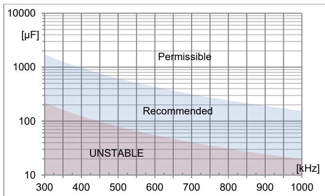
Effective total output capacitance limits vs switching frequency.
