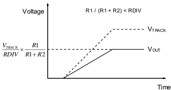
Ratiometric Voltage Tracking
