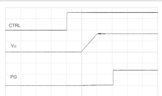
Start-up enabled by CTRL signal. T_{ON\_DELAY} = T_{ON\_RISE} = 10\text{ ms} (default). V_i = 12\text{ V} , I_o = \text{max } I_o , PG pulled up to V_o . Scale: 2 V/div, 10 ms/div.
