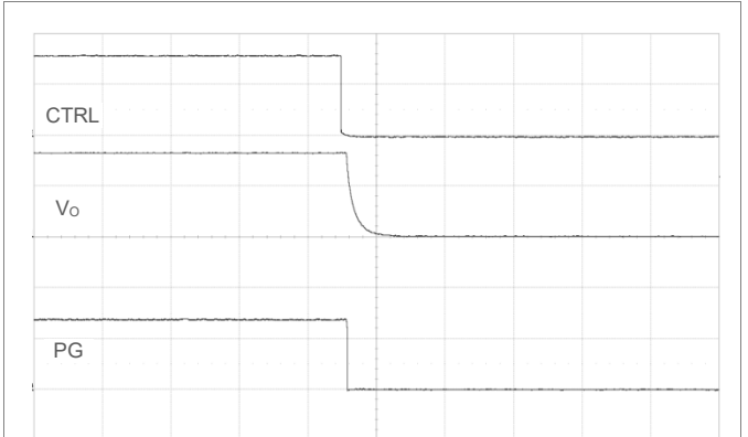
Shut-down by CTRL signal. V_i = 12\text{ V} , I_o = \text{max } I_o , PG pulled up to \bar{V}_O . Scale: 2 V/div, 1 ms/div.
