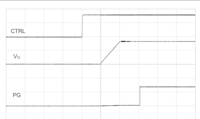
Start-up enabled by CTRL signal. T_{ON\_DELAY} = T_{ON\_RISE} = 10\text{ ms} (default). V_i = 12\text{ V} , I_o = \text{max } I_o , PG pulled up to \bar{V}_O . Scale: 2 V/div, 10 ms/div.
