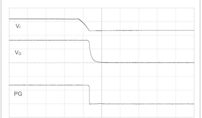
Shut-down by removing V_i . V_i = 12\text{ V} , I_o = \text{max } I_o , PG pulled up to \bar{V}_O . Scale: 10 or 2 V/div, 1 ms/div.
