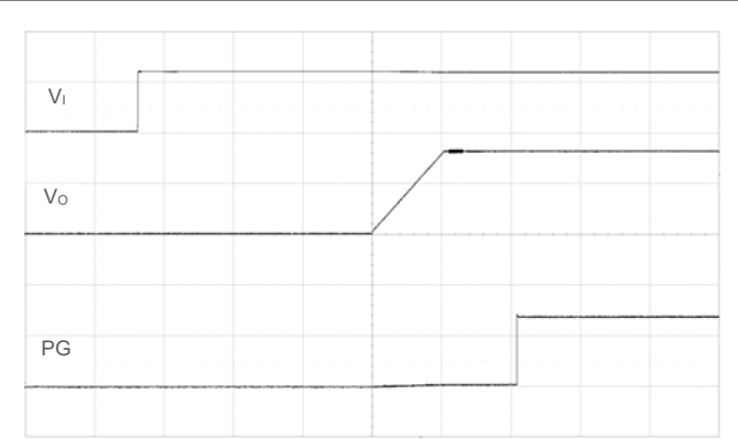
Start-up enabled by applying V_i . T_{ON\_DELAY} = T_{ON\_RISE} = 10\text{ ms} (default). V_i = 12\text{ V} , I_o = \text{max } I_o , PG pulled up to V_o . Scale: 10 or 2 V/div, 10 ms/div.
