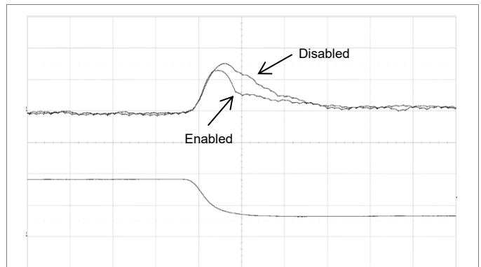
Recovery time to within 1% of V_O vs. ZETAP setting.
