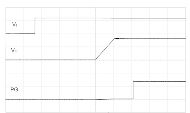
Start-up enabled by applying V_i . T_{ON\_DELAY} = T_{ON\_RISE} = 10\text{ ms} (default). V_i = 12\text{ V} , I_o = \text{max } I_o , PG pulled up to \bar{V}_O . Scale: 10 or 2 V/div, 10 ms/div.
