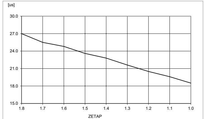
Recovery time to within 1% of V_O vs. ZETAP setting.
