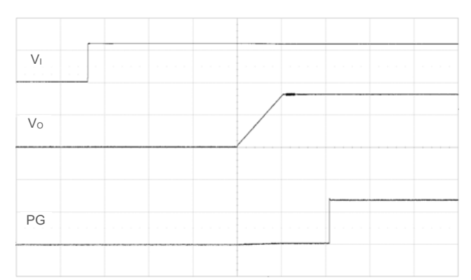
Start-up enabled by applying V_i . T_{ON\_DELAY} = T_{ON\_RISE} = 10\text{ ms} (default). V_i = 12\text{ V} , I_o = \text{max } I_o , PG pulled up to V_o . Scale: 10 or 1 V/div, 10 ms/div.
