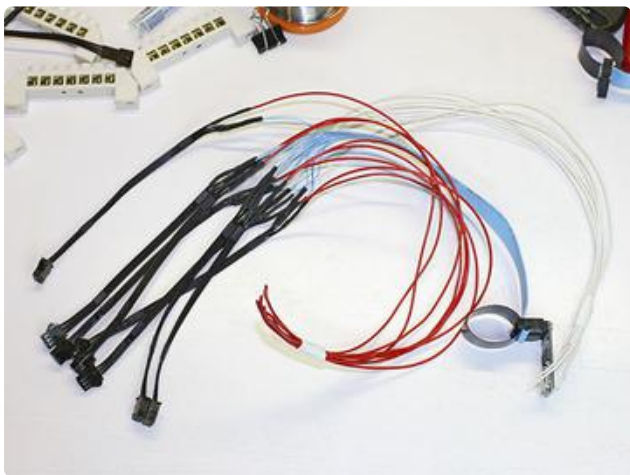
Here's one of the wiring harnesses nearly complete. The 18 gauge power pigtails haven't yet been added.
