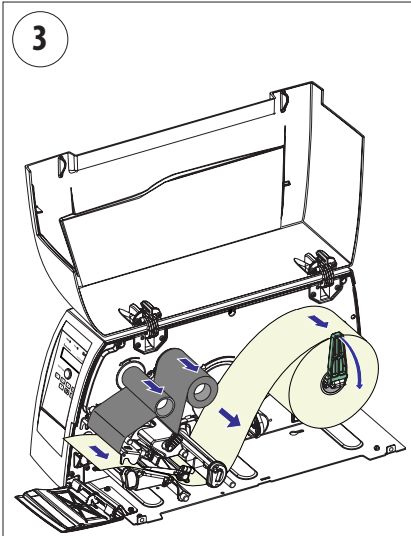
Remove any media and transfer ribbon.
