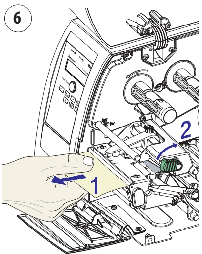
Pull out the cleaning card (1) and raise the printhead (2).
