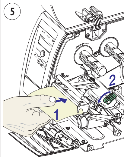
Insert most of the cleaning card under the printhead (1). Engage the printhead (2).
