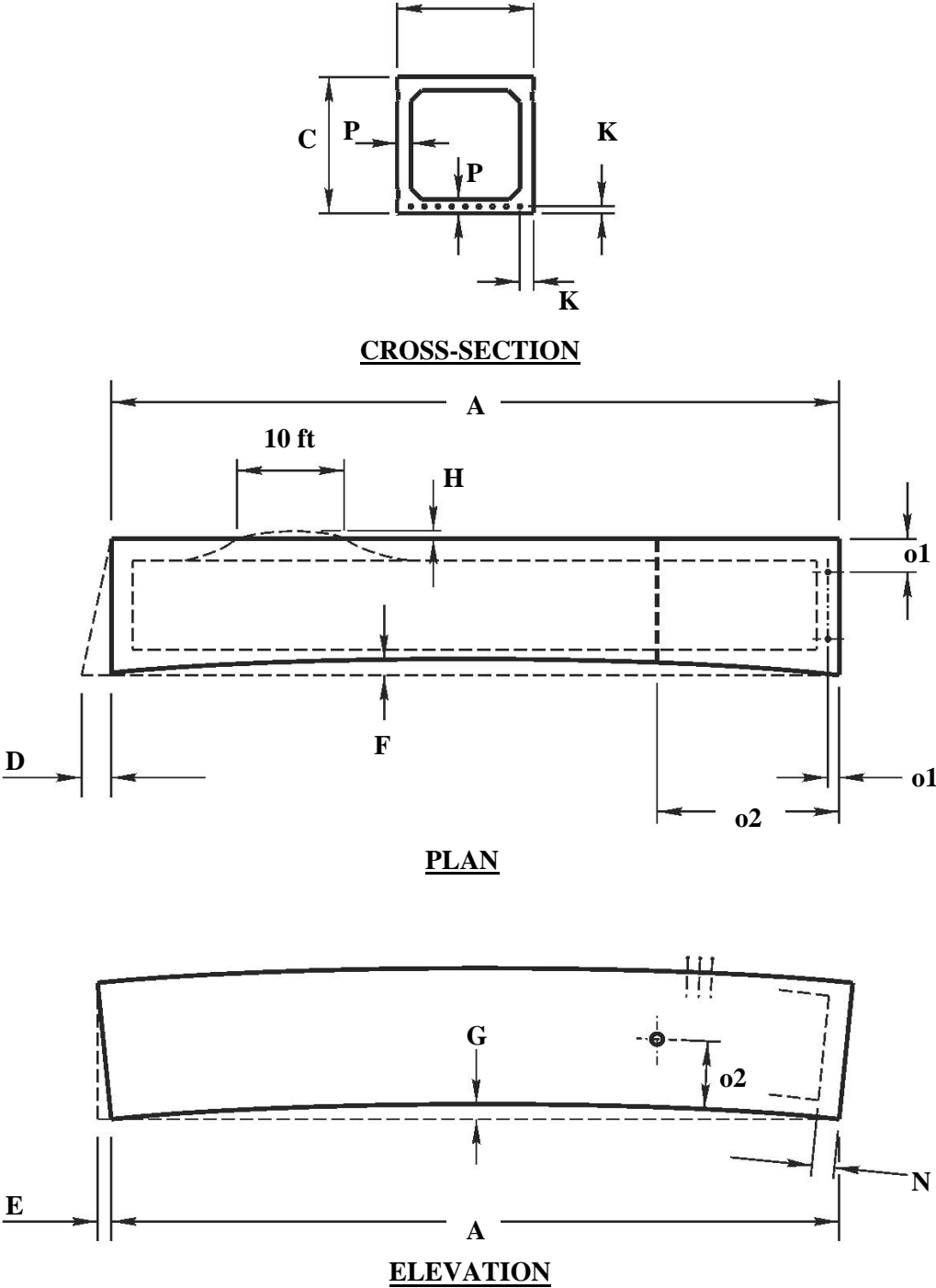
1 Figure 1078-4. Prestressed Box Beams. Dimensions shown are in Table 1078-7.
