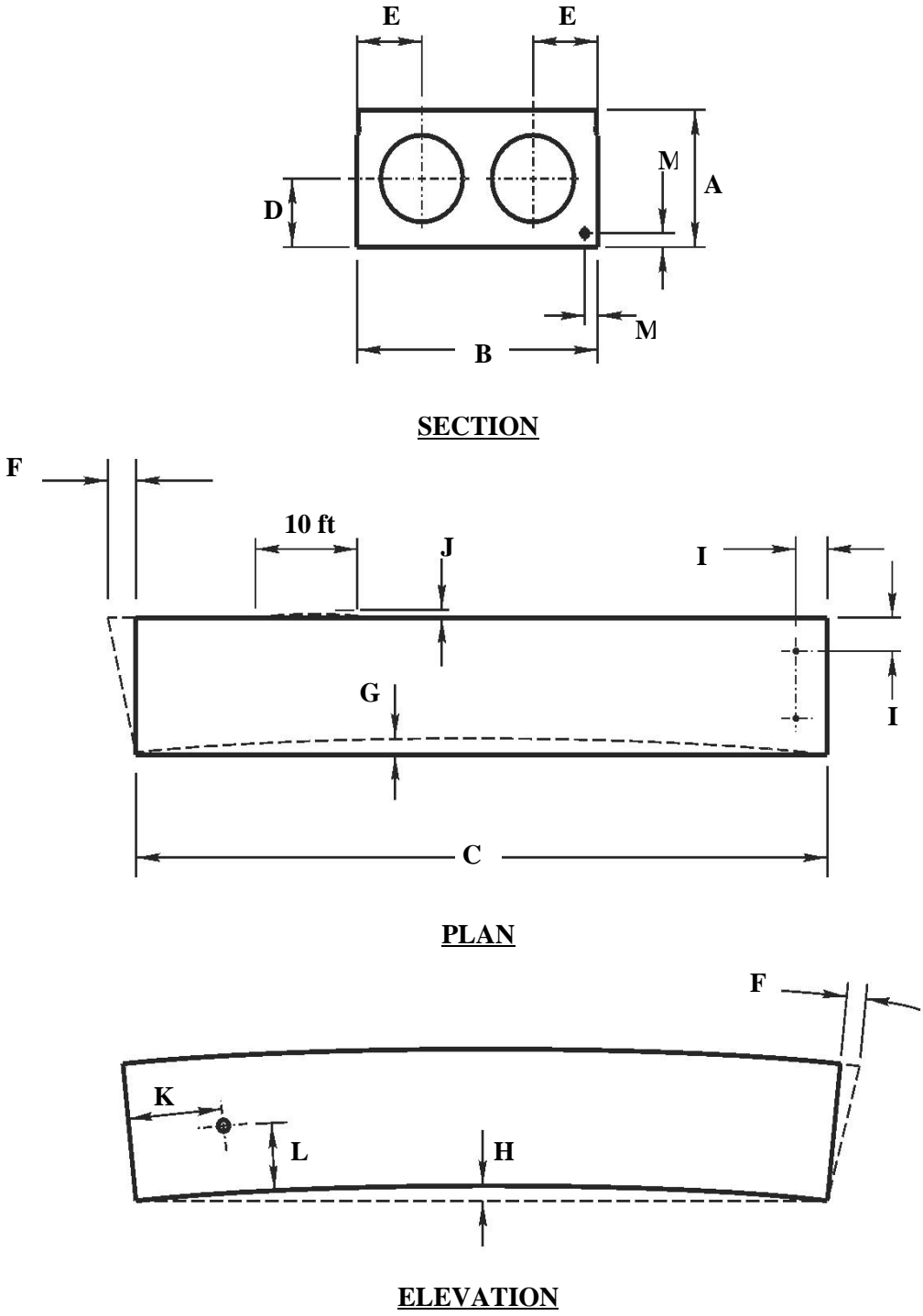
1 Figure 1078-2. Prestressed cored slabs. Dimensions shown are in Table 1078-4.
