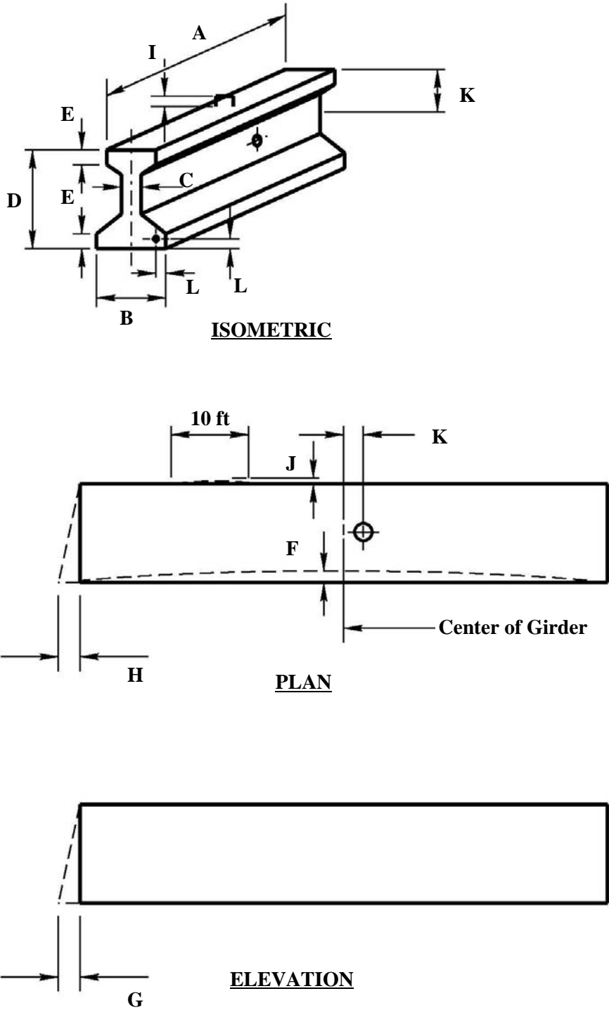
1 Figure 1078-3. Prestressed Girders. Dimensions shown are in Table 1078-5.
