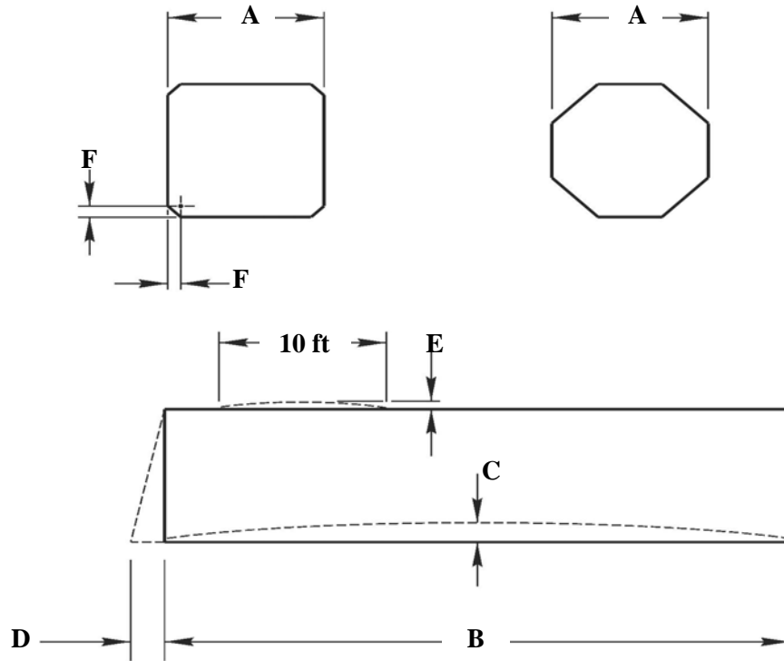
7 Figure 1078-1. Prestressed Piles. Dimensions shown are in Table 1078-3.
