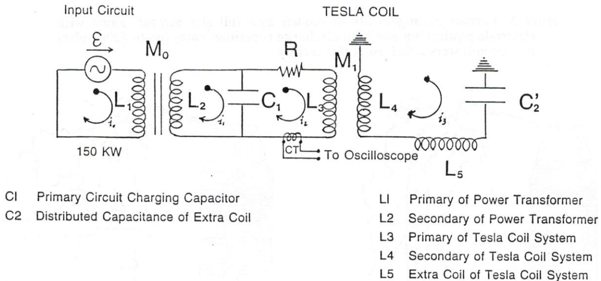
Figure 3. Equivalent circuit of Golka Associates Tesla Coil.
