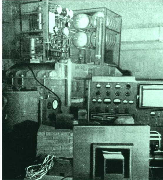
Armenian Hydro-Magnetic Dynamo in its Protective Plastic ‘Jacket’
