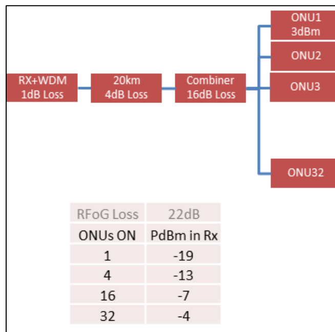
Figure 4 – Illustrating Optical Rx Dynamic Range
