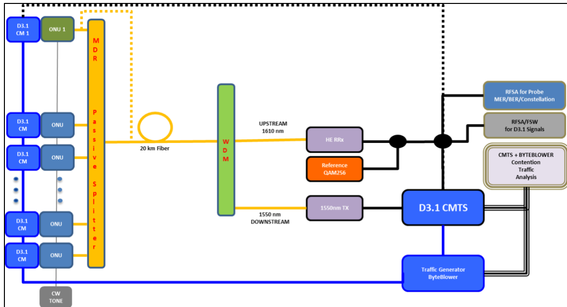
Figure 15 – 16 CM/ONU System Configuration
