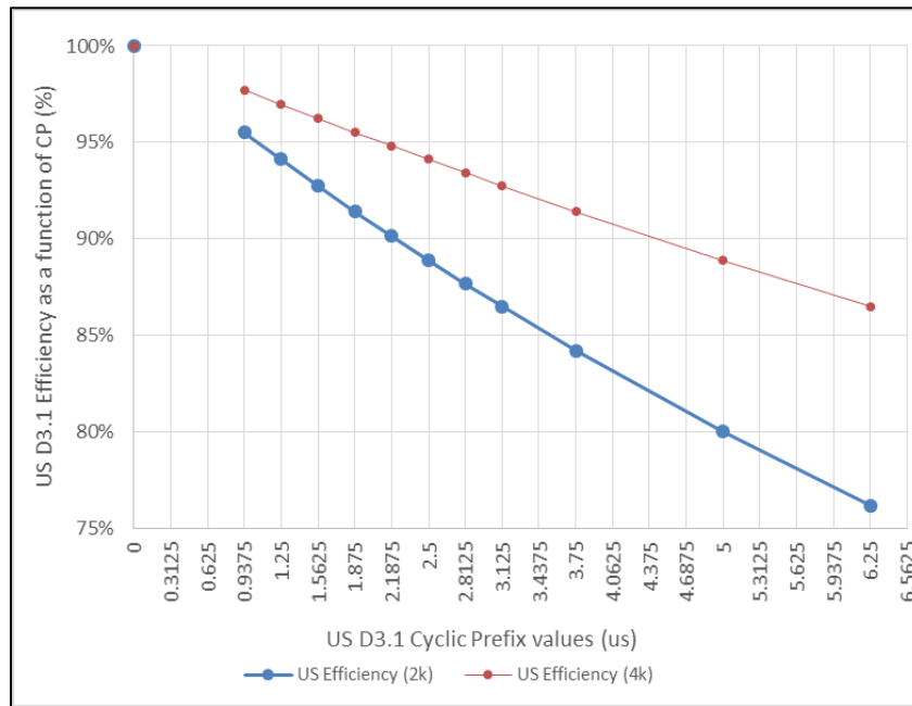
Figure 2 – US DOCSIS 3.1 Efficiency as a Function of Cyclic Prefix
