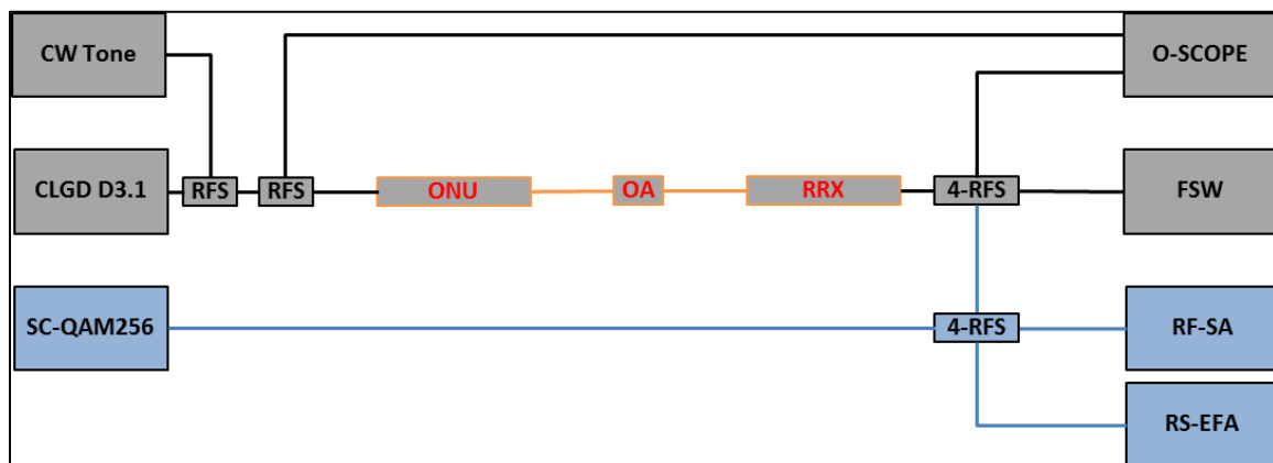
Figure 9 – CLGD-FSW Single ONU Test Set-up
