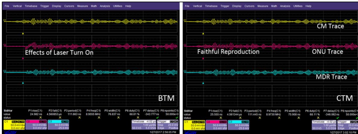
Figure 12 – Time Domain Capture of the Effects of the Laser Turn On
