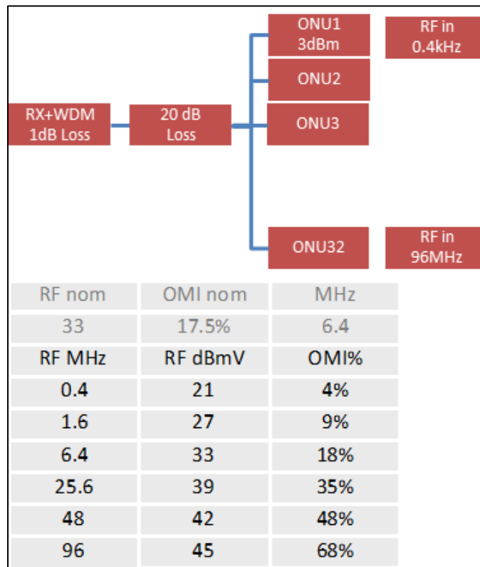
Figure 5 – Illustrating ONU RF Input Dynamic Range
