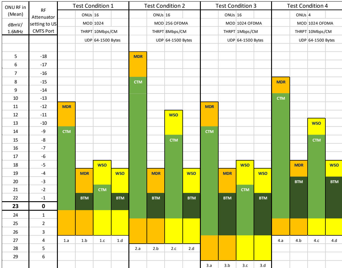
Figure 17 – Measured System Dynamic Slivers and Dynamic Ranges
