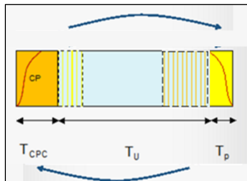
Figure 1 – Illustrating the DOCSIS 3.1 US Symbol and CP, RP
