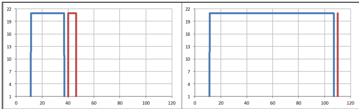
Figure 6 – Illustrating Typical RF Levels: DOCSIS 3.0 Left and DOCSIS 3.1 Right
