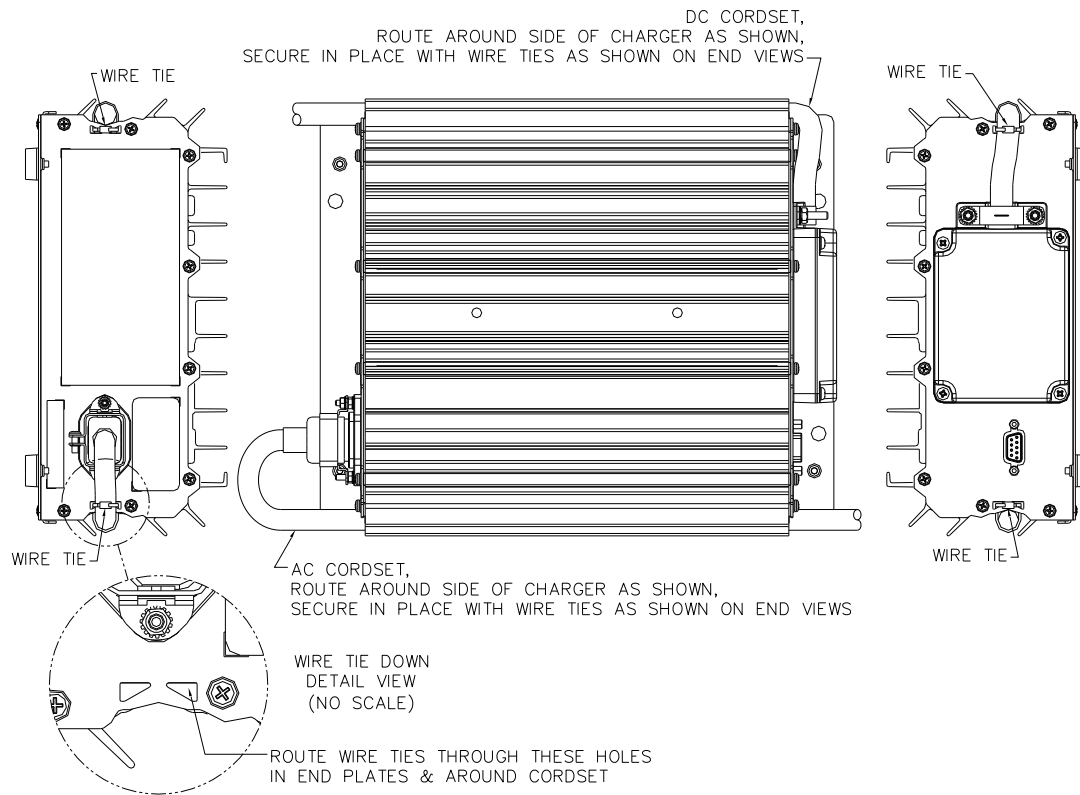
Figure 2-3: AC & DC Cordset Routing
