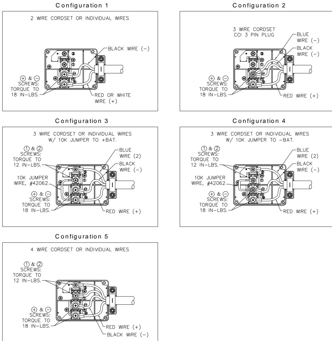
Figure 6.2-2: DC Terminal Block Configurations
