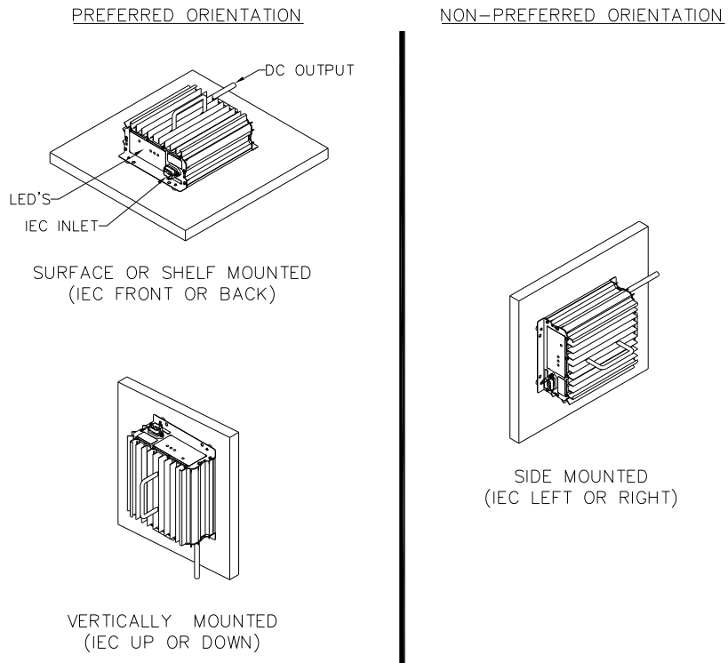
Figure 2-1: Charger Mounting Recommendations
