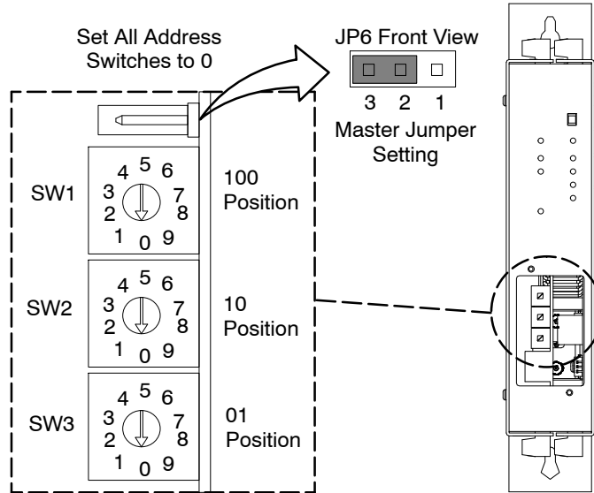
Figure 2 Factory Settings for Address Switches and JP6 Jumper Setting
