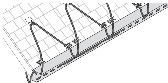
Roof and gutter de-icing: standard roof
