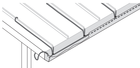
Roof and gutter de-icing: standing seam metal roof
