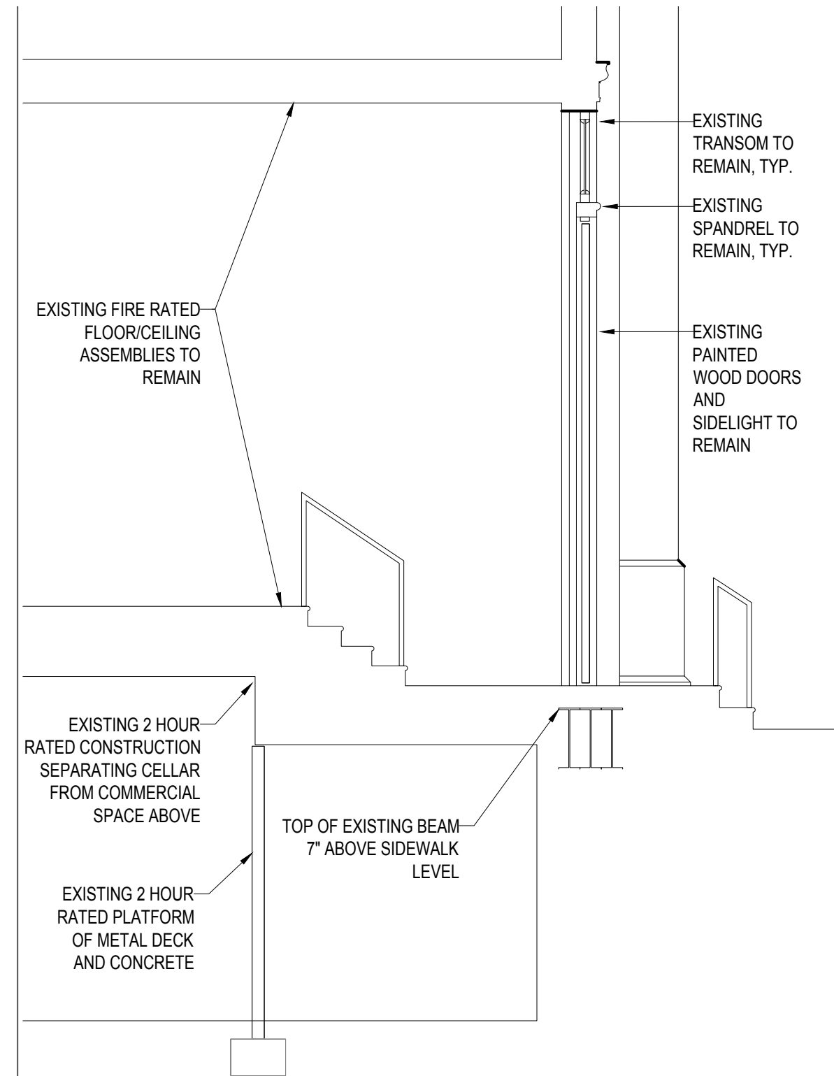
RETAIL LOBBY SECTION
