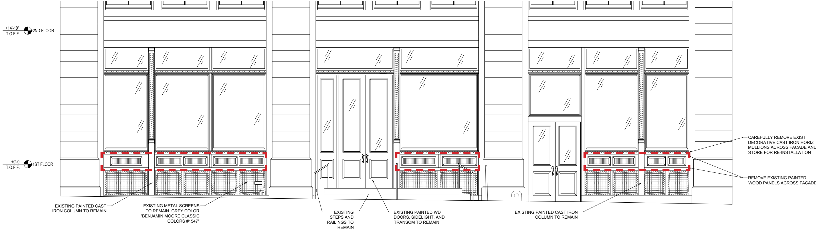
84 WOOSTER STREET EXISTING STOREFRONT ELEVATION
