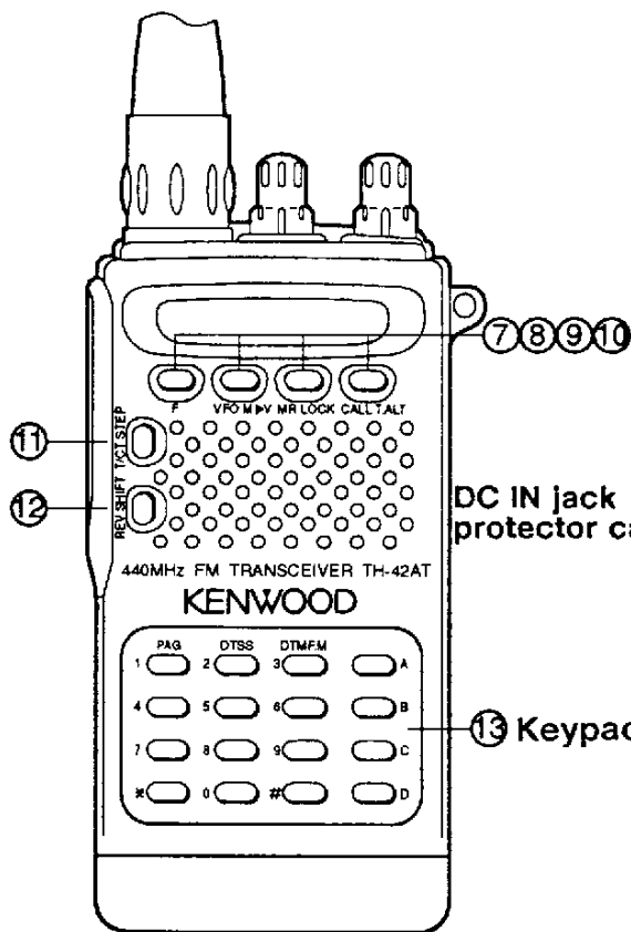
TH-42AT The keypad is an option for General market versions.
