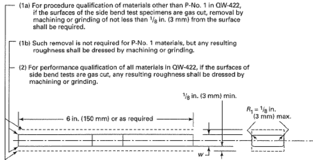
QW-462.2 SIDE BEND
