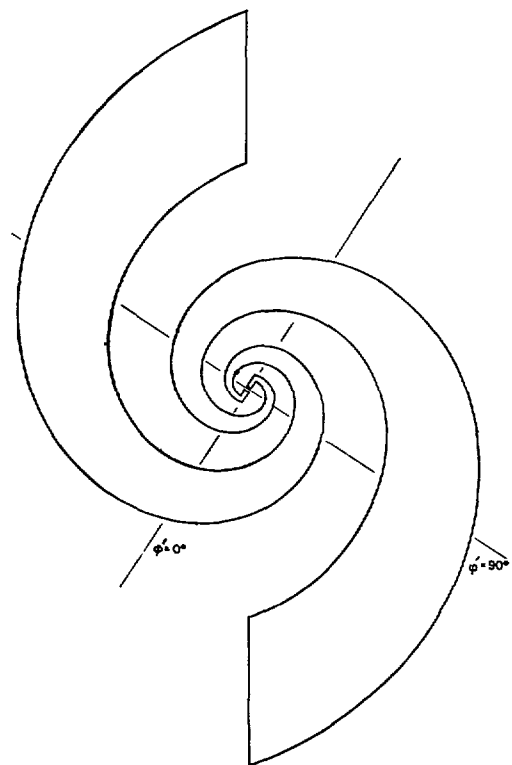
Fig. 2—Outline drawing of an antenna. ( a=0.35 , K=0.597 , k=0.2 inch, maximum diameter = 9 \frac{3}{16} inch.)
