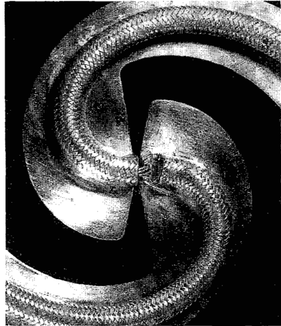
Fig. 4—Terminal region of antenna shown in Fig. 3(b).
