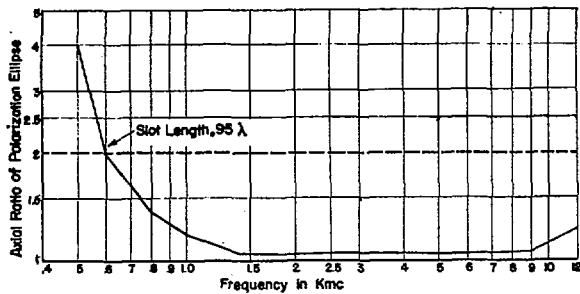
Fig. 5—Polarization, on axis, of the radiated E field of antenna shown in Fig. 3(a).
