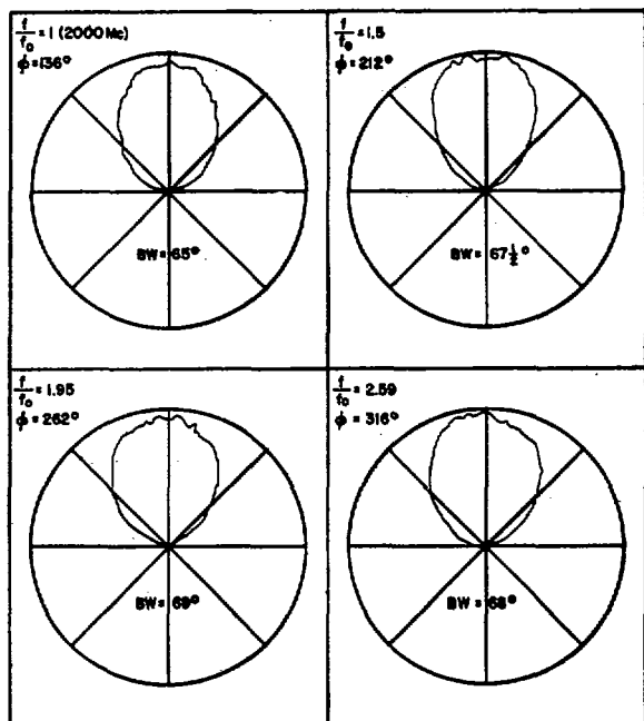
Fig. 11—Patterns obtained by simultaneous rotation of antenna and increase in frequency. ( a=0.303 , K=0.75 , k=0.2 inch, L=33 cm) \phi polarization.
