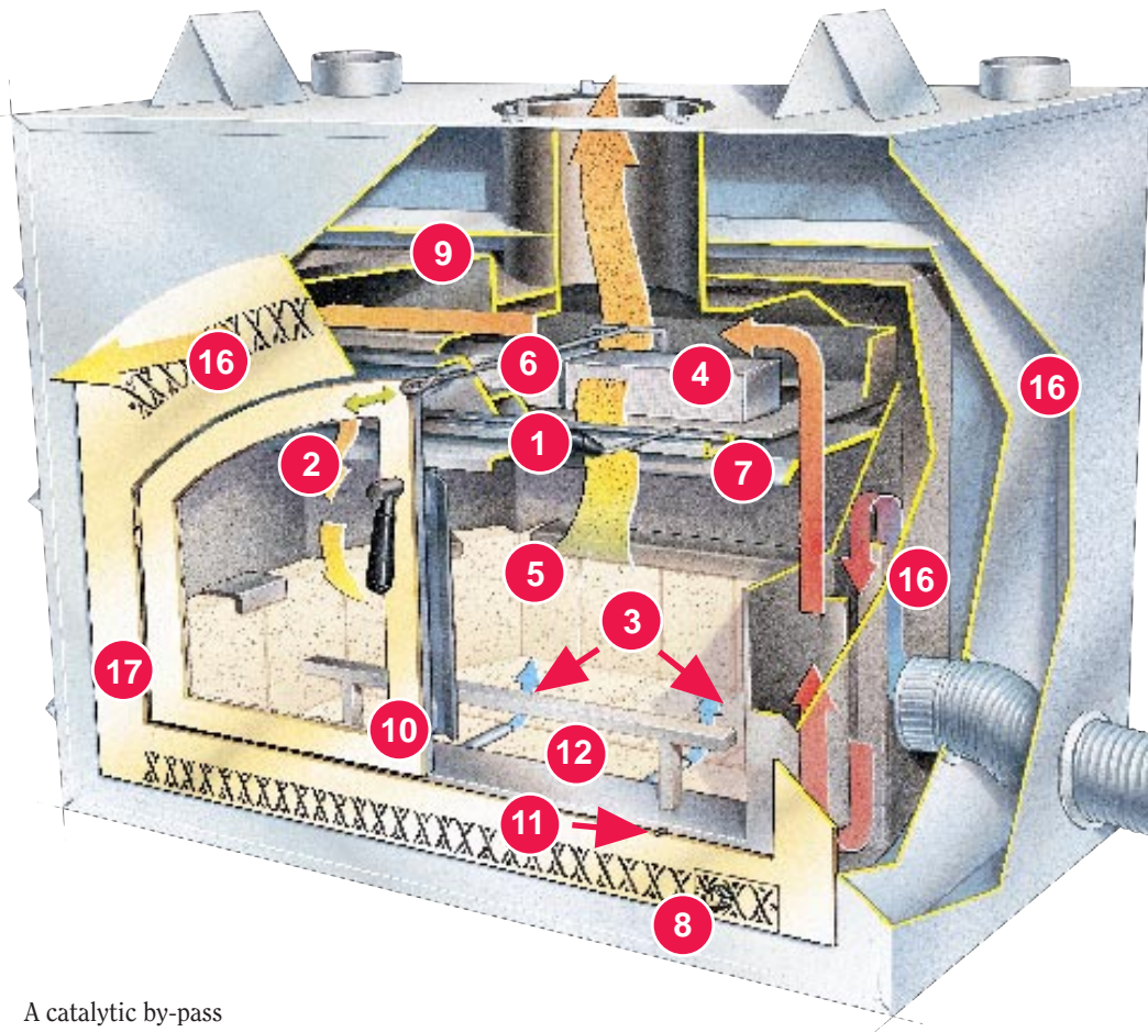
Model 36 Elite Zero Clearance Fireplace
