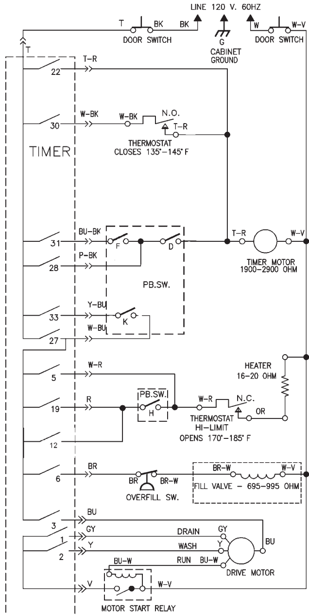
Wiring Diagram
