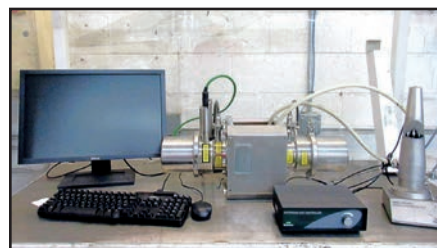
MALVERN RT SIZER LASER PARTICLE SIZE ANALYZER
