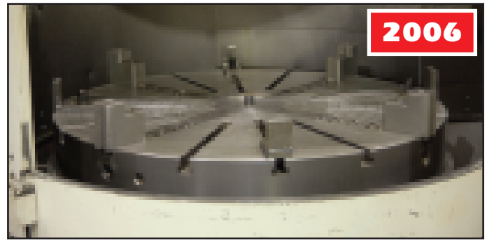
59" 4-JAW CHUCK FOR 2006 TOSHIBA TUE-15 VERTICAL BORING MILL
