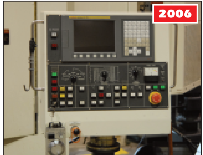
FANUC SERIES 0I-TC CONTROL FOR 2006 TOSHIBA TUE-15 VERTICAL BORING MILL
