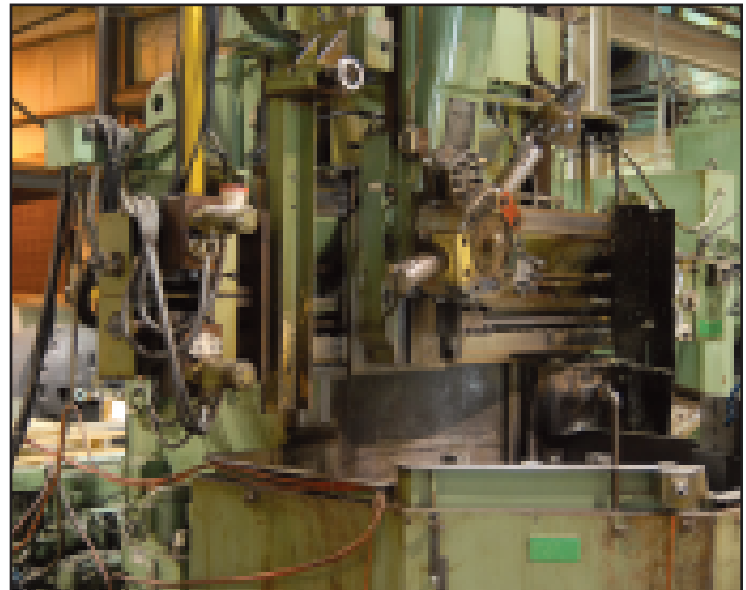
MIMIK HYDRAULIC TRACER ON BULLARD 52" VERTICAL TURRET LATHE
