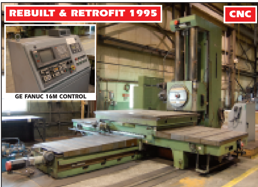
SCHARMANN 80" X 100" T-SLOTTED ROTARY TABLE TYPE CNC HORIZONTAL BORING MILL
