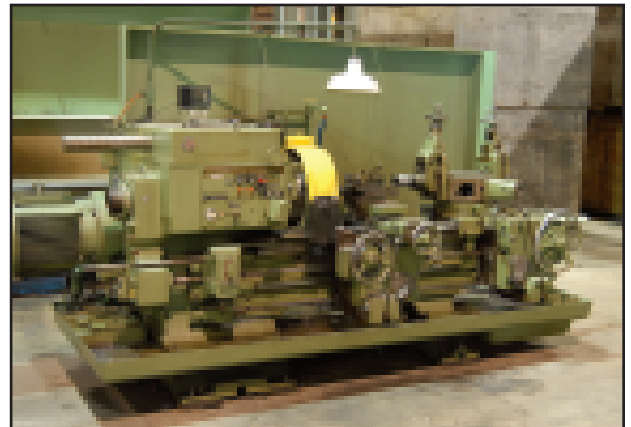
WARNER AND SWASEY #2A SQUARE HEAD TURRET LATHE
