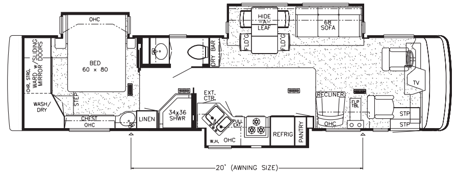
Model Shown: KSDP3904
