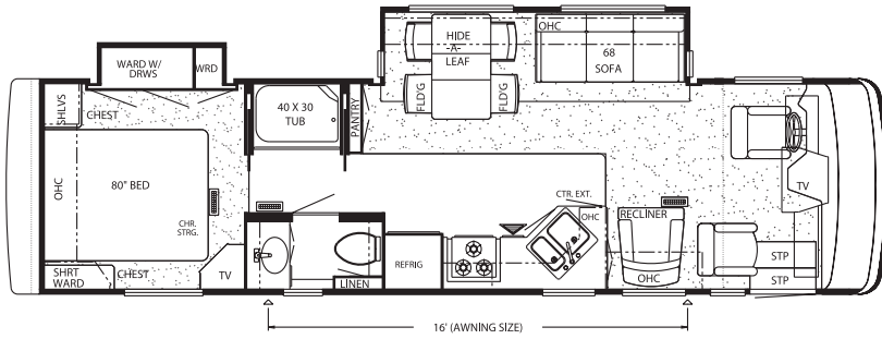
Model Shown: KSDP3353
