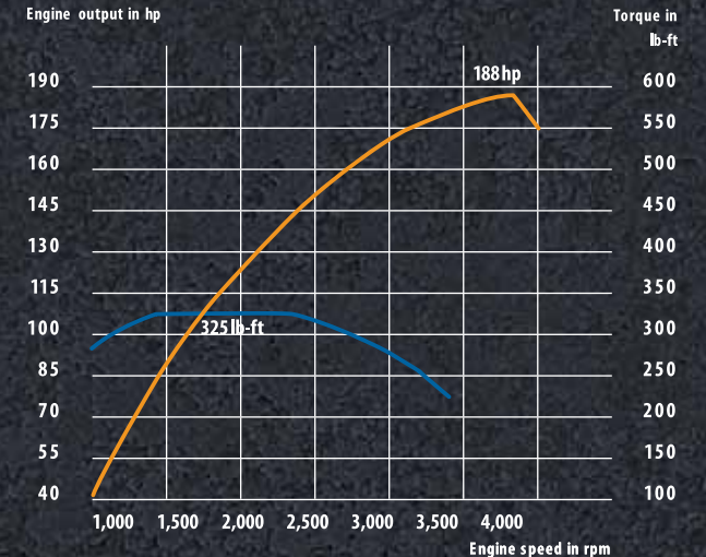
Torque curve: Engine output in hp
