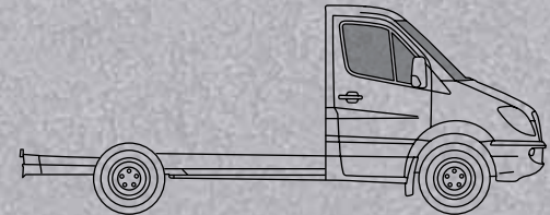
144" WHEELBASE – 2500 CARGO / CREW / PASSENGER – 8,550 LBS GVWR
