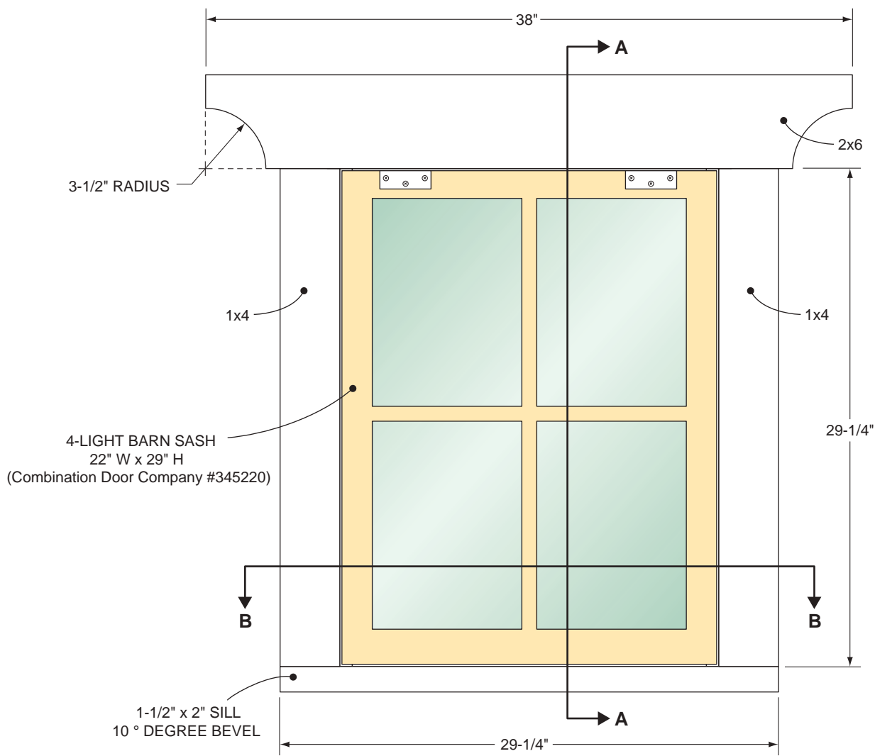
Figure M Pre-hung Barn Sash Construction
