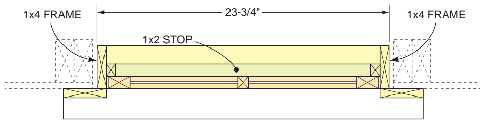
SECTION B-B
