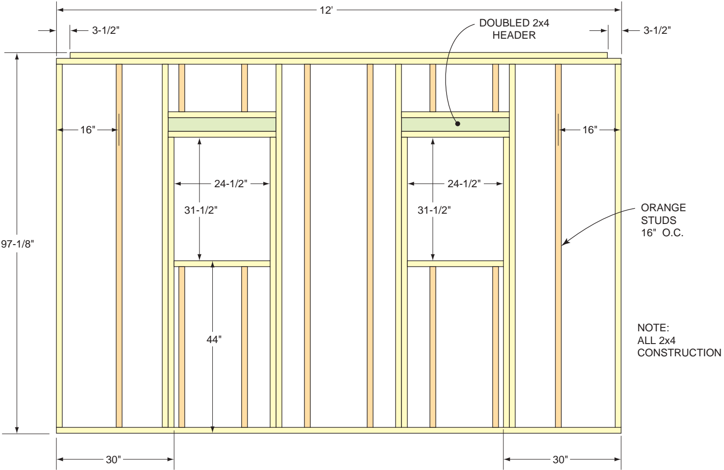
Figure D Side Walls Framing and Siding
