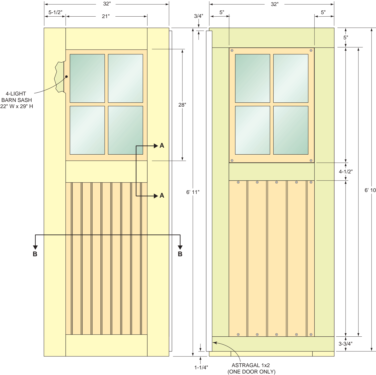
Figure N Site-built Door Construction
