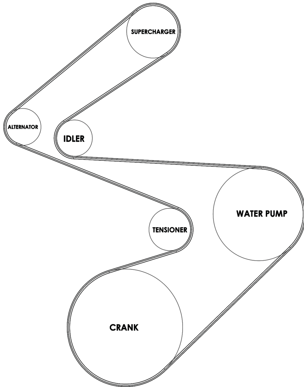
Belt Routing Diagram
