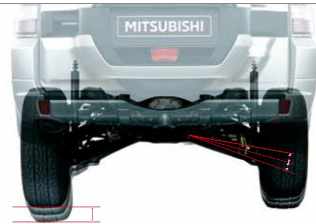
Each wheel can raise, lower and pivot independently, keeping more tire surface against the ground for greater stability
