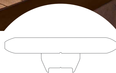
CONTEMPORARY RAIL TOP RAIL SIZE: 6.4" X 3"
