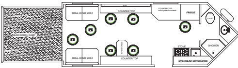
18THEXP | Cargo Length 10' (10 3 / 8 "")
