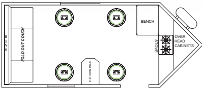
12 RC with Rear Sofa
