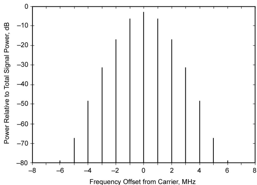
Figure 4. Spectrum for Sinewave Range Component; 1 MHz with \phi_r = 0.80 rad rms
