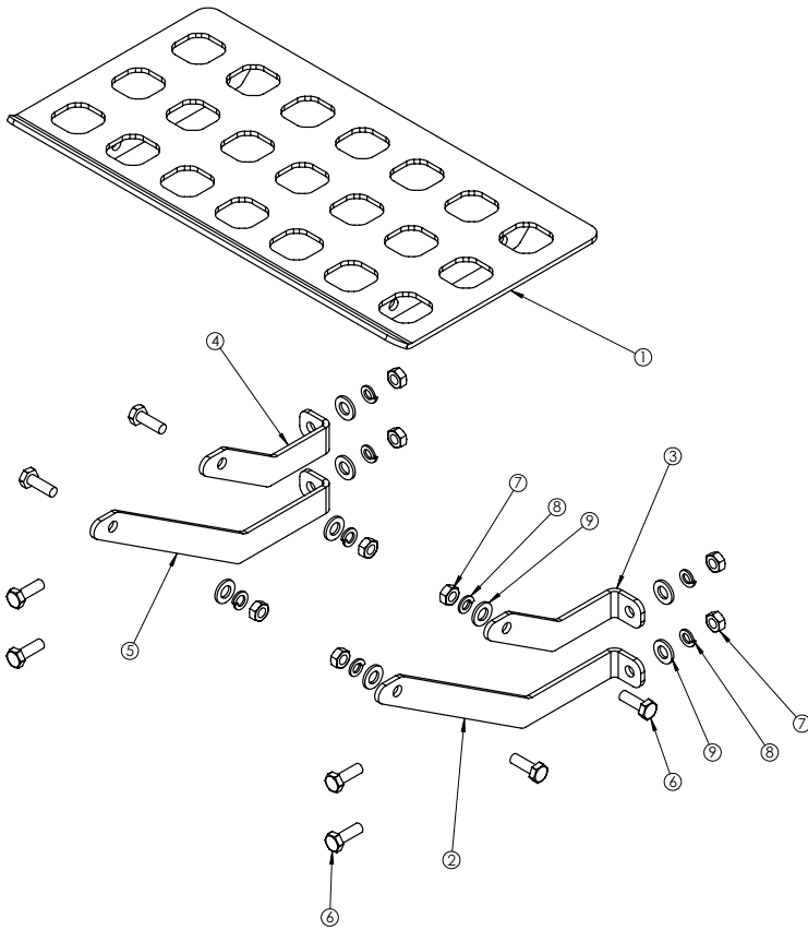
101392 Log Catcher Assembly For 25-Ton
