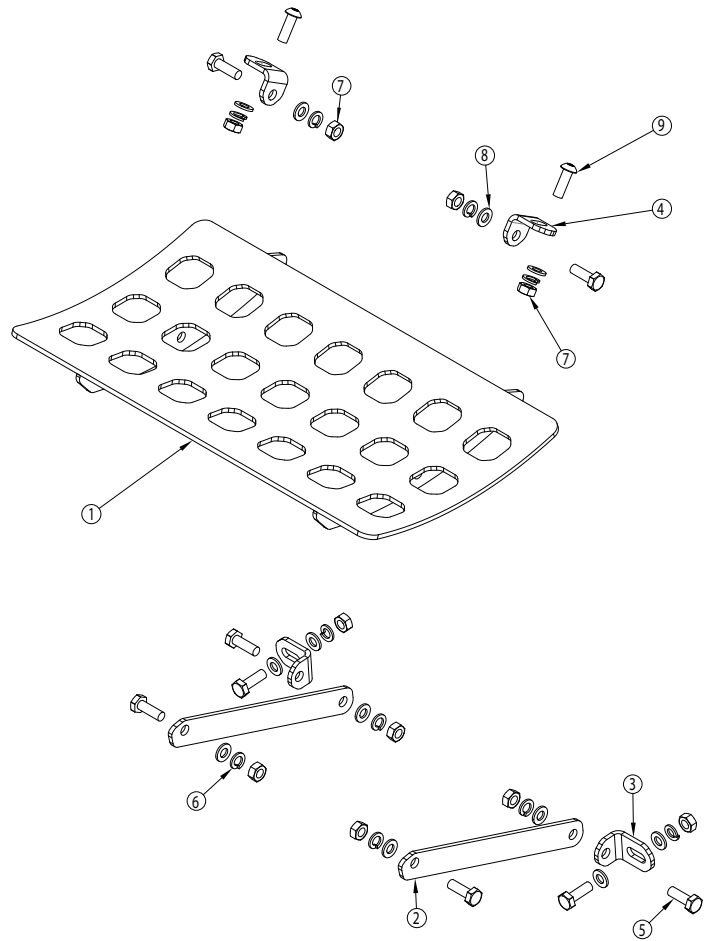
100173 Log Catcher Assembly For 30-Ton
