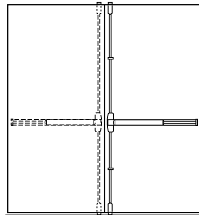
Two vertical cables/rods—double egress
