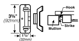
Projection 1 5/16" (21mm)
