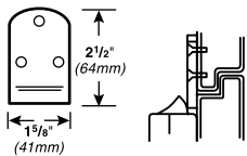
Projection 3/8" (10mm)
