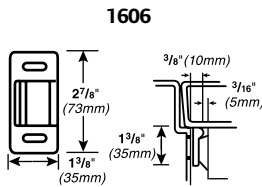
Projection 3/8" (10mm)
