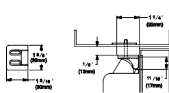
Projection 1 1/4" (32mm)
