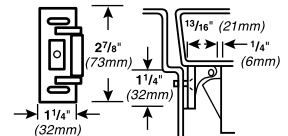
Projection 1 3/16" (21mm)
