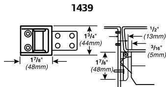
Projection 1/2" (13mm)
