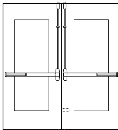
Two FEH vertical cable/rods with auxiliary fire latch-LBR option
