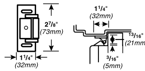
Projection 1 3/16" (21mm)
