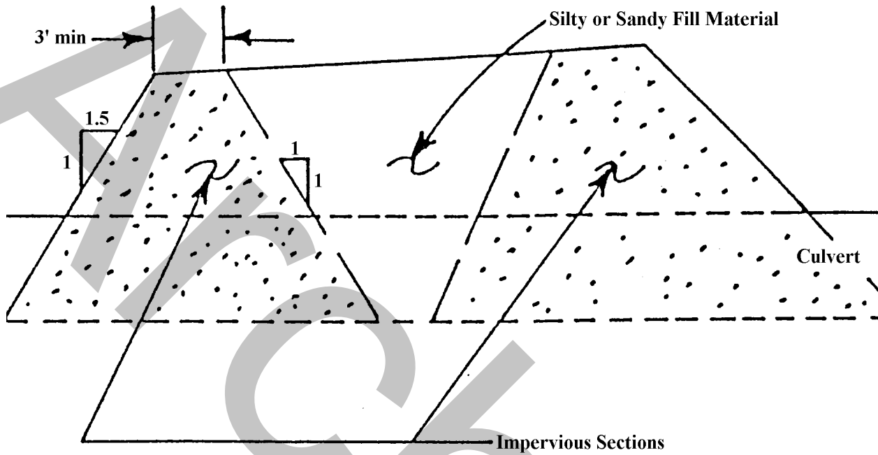
FIGURE 19. Culvert Backfill Using Silty or Sandy Material
