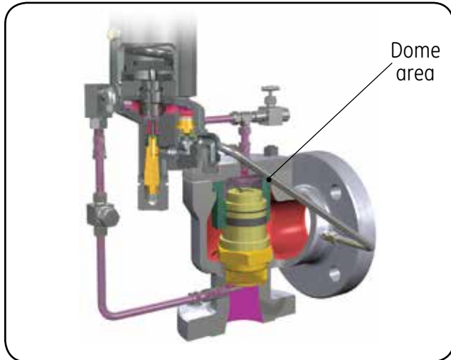
MV Valve Closed (Normal Position)
