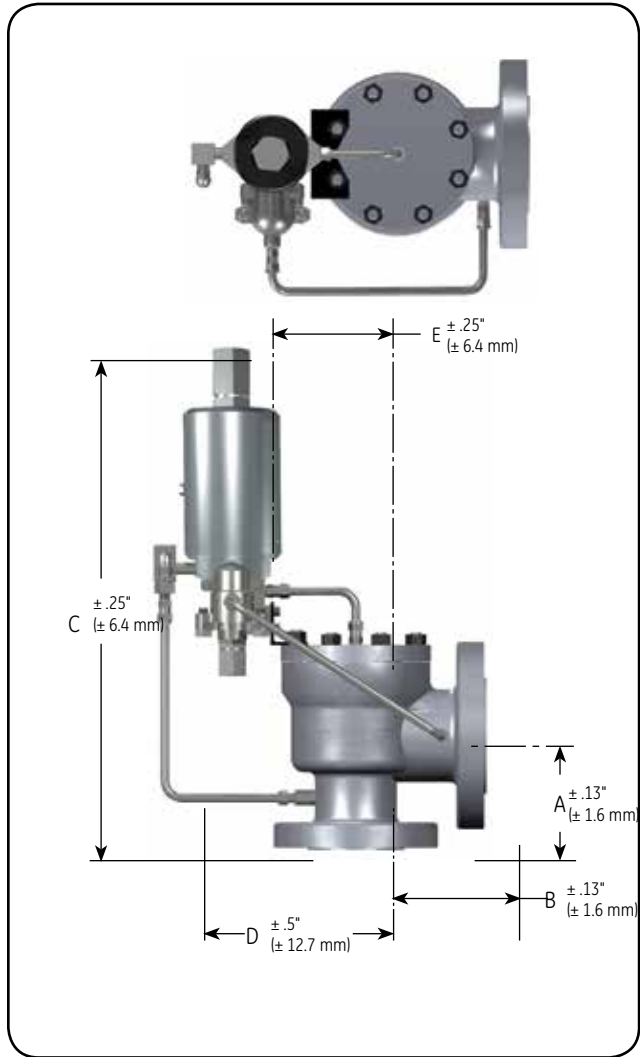
39MV with Single Outlet - Full Bore
