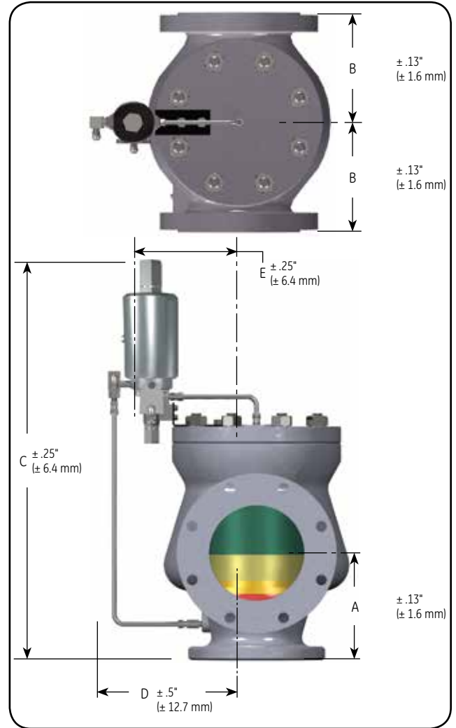
39PV with Double Outlet - Full Bore
