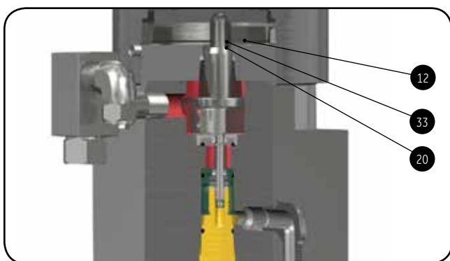
39MV72 Pilot Construction
