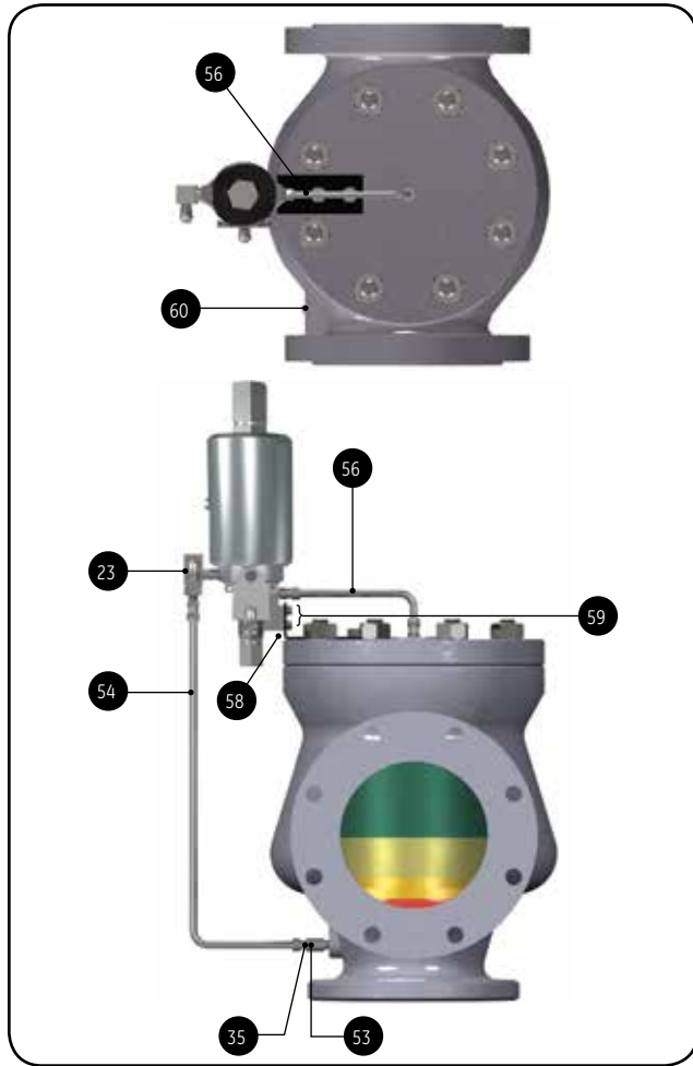
Pilot Valve with Field Test Connection (Standard For All Media Applications)
