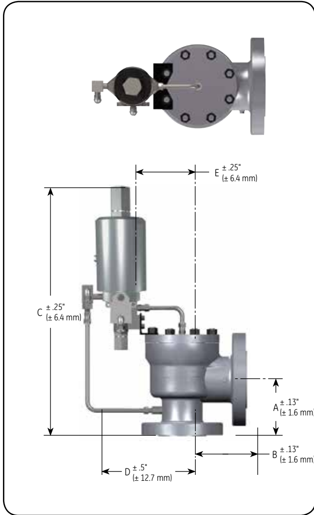
39PV with Single Outlet - Full Bore
