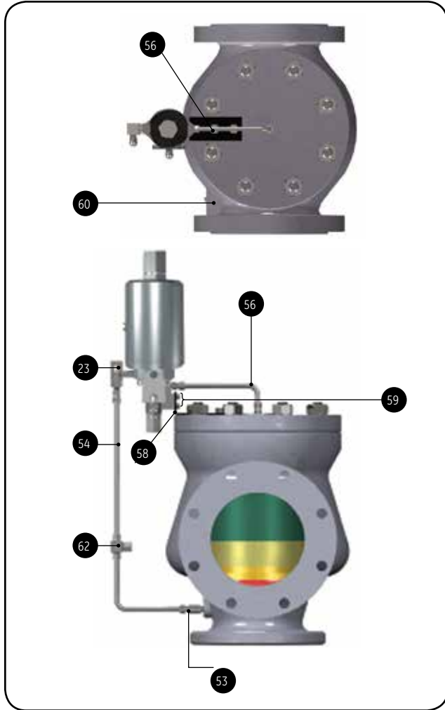
Pilot Valve with Pilot Supply Filter (Optional For All Media Applications)
