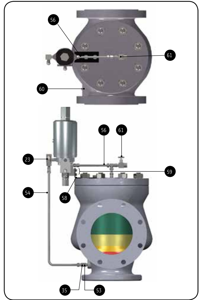
Pilot Valve with Manual Blowdown (Optional For Liquid and Gas Applications)
