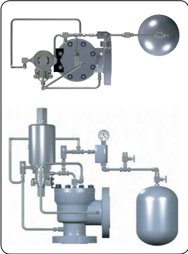
Pilot Valve Tester
