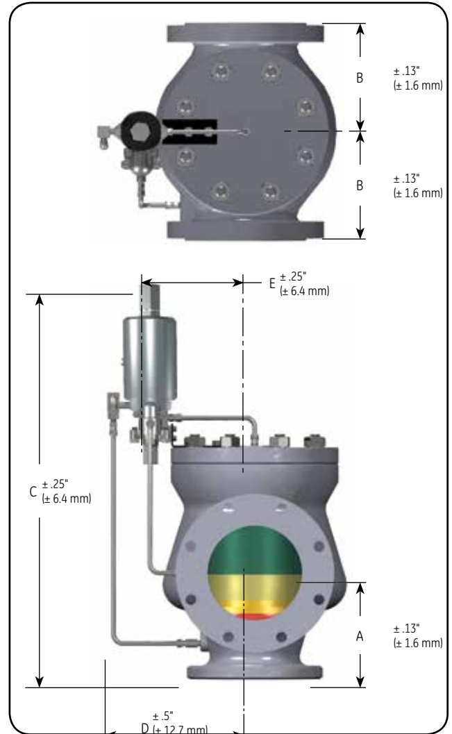
39MV with Double Outlet - Full Bore
