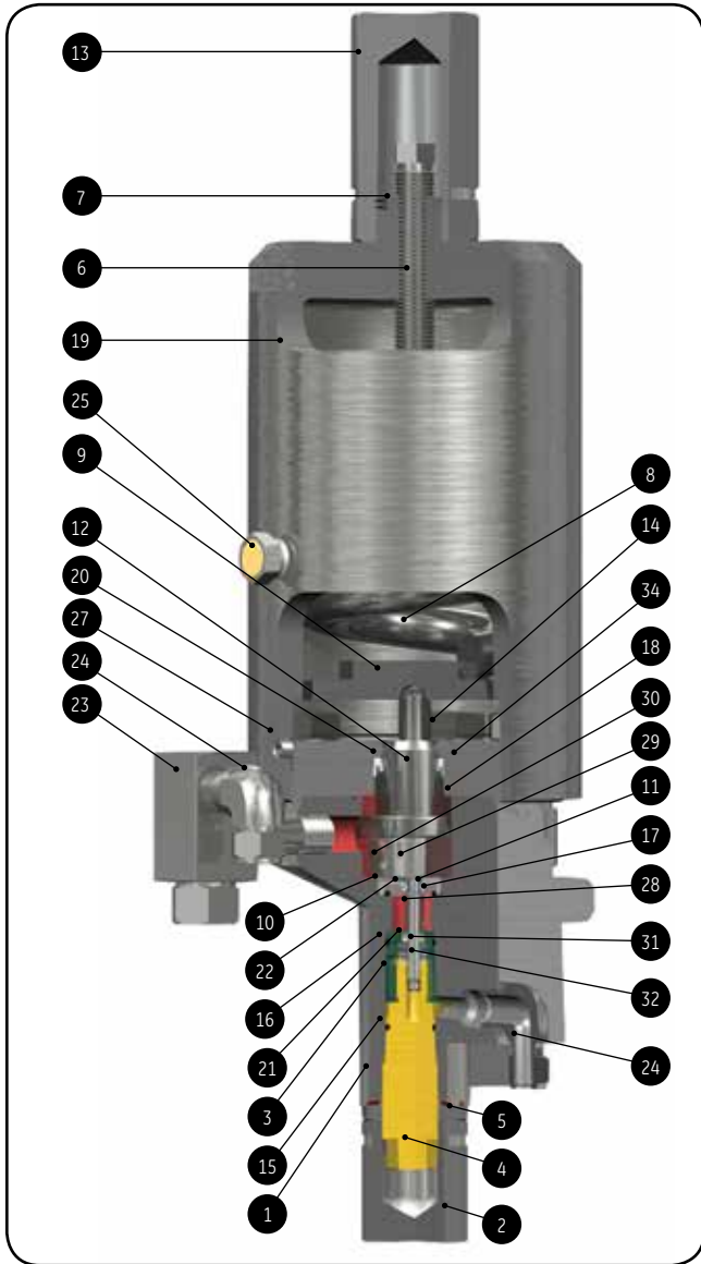
39MV72 Pilot Construction
