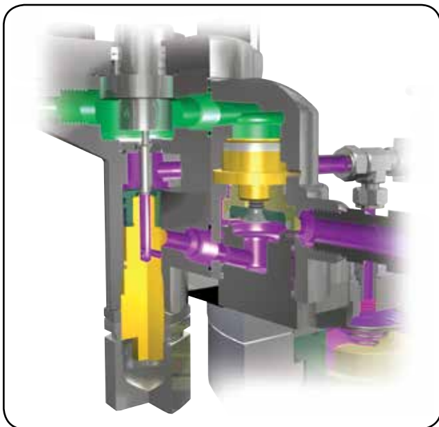
MV Fully Open
