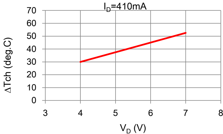
\Delta T_{ch} vs. V_D Voltage (Reference)
