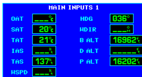
Figure 5-6. MAIN INPUTS 1 Page
