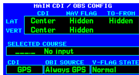
Figure 5-14. MAIN CDI/OBS CONFIG Page
