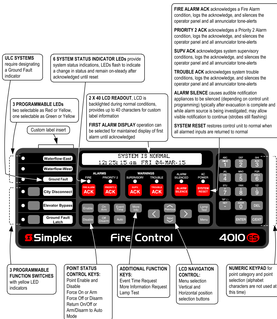
Figure 2: Operator Interface Features
