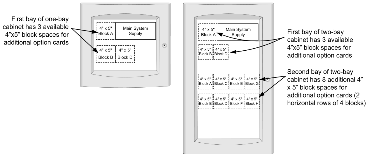
Figure 3: Loading Reference
