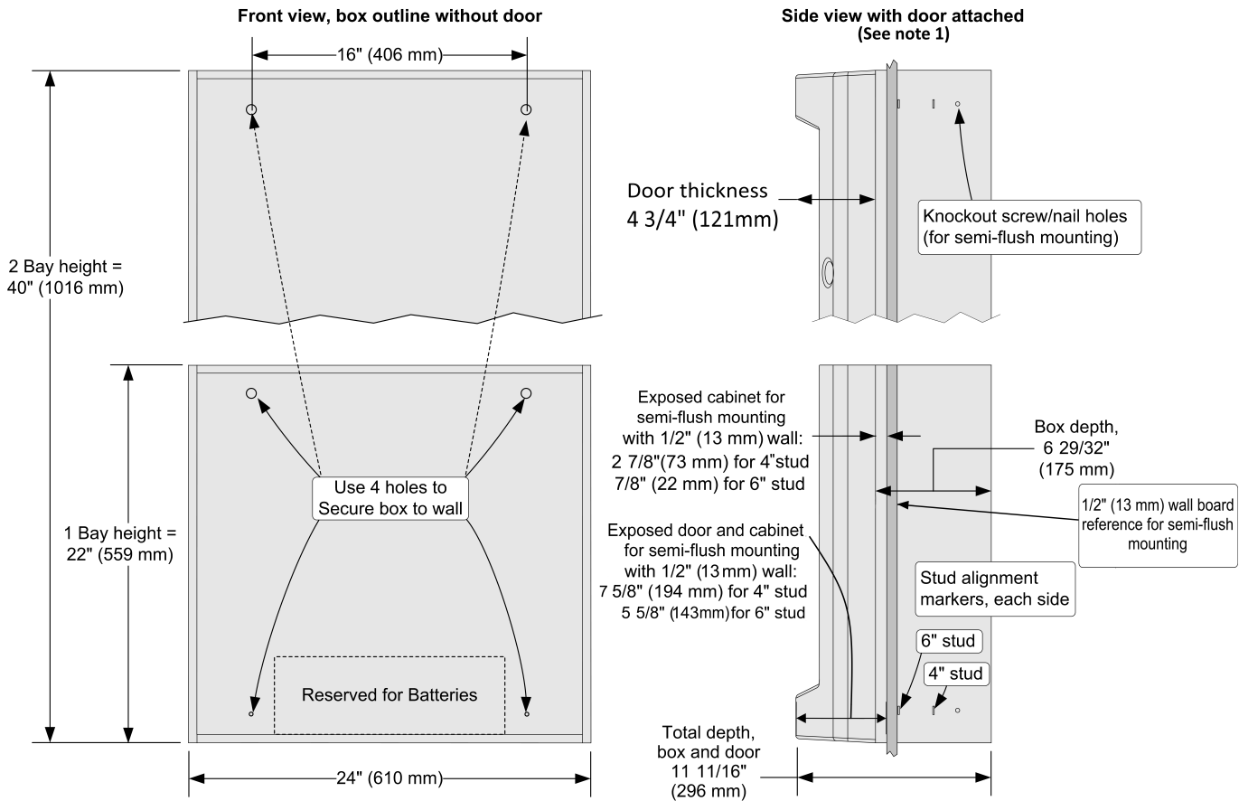
Figure 4: Cabinet Dimension Reference
