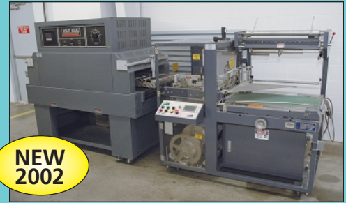
Overall View Hangata Heat Shrink and L-Seal System
