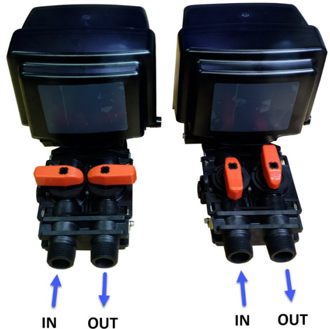
5900 VALVE BY-PASSED
