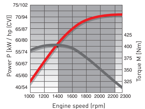
QUANTUM C POWER CURVE
