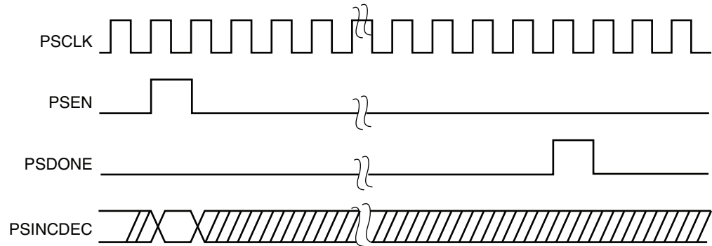
Figure 3-7: Phase-Shift Timing Diagram
