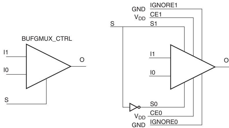
Figure 2-13: BUFGMUX_CTRL as BUFGCTRL
