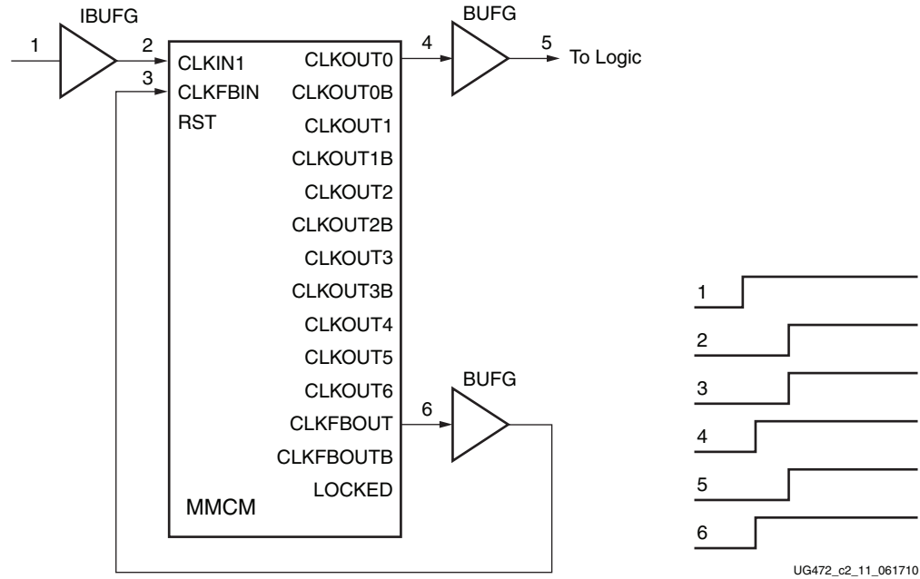
Figure 3-11: Global Clock Network Deskew Using Two BUFGs
