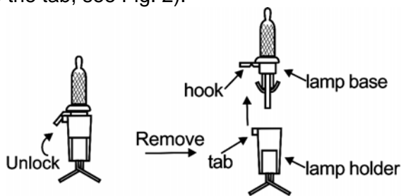
Fig.1 Unlock and remove the burned out lamp
