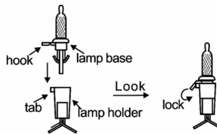
Fig.2 Replace with the spare lamp
