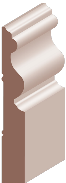
#193 9/16 X 4-1/2 "175" BASE
