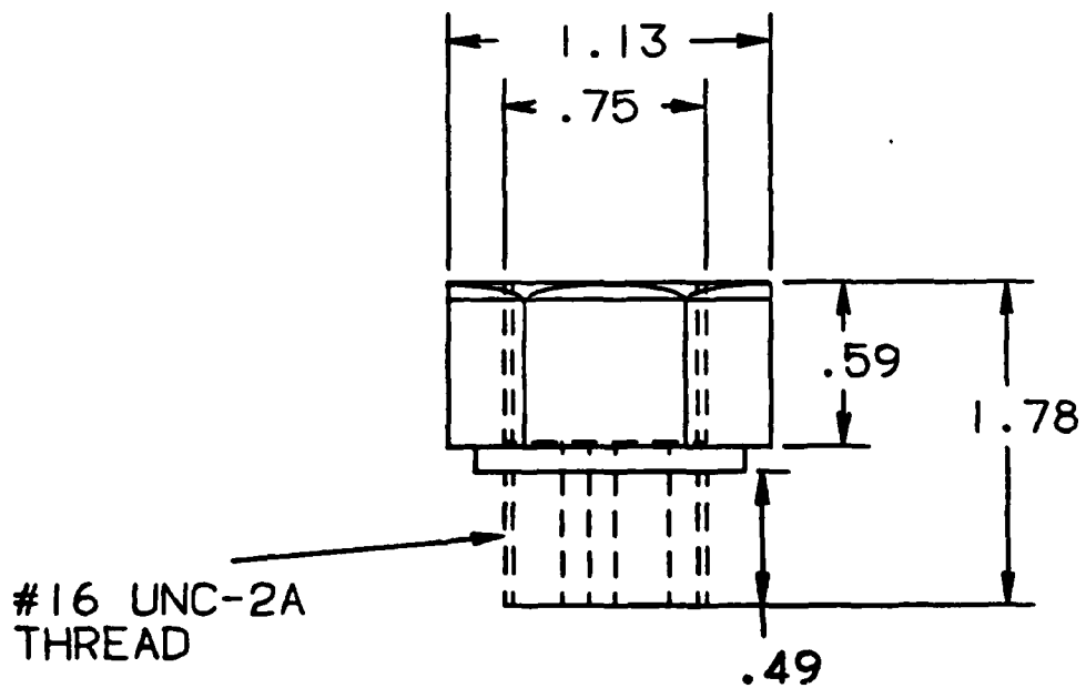
Figure 6. Housing of the prototype shear pressure gauge.
