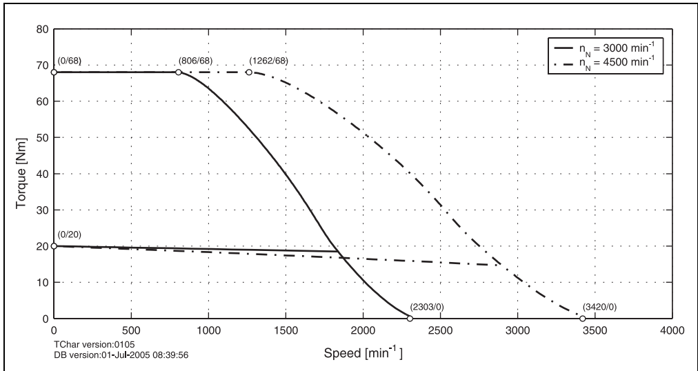
Figure 46: Speed - torque characteristic curve for 8LSA64.eennnffgg-0
