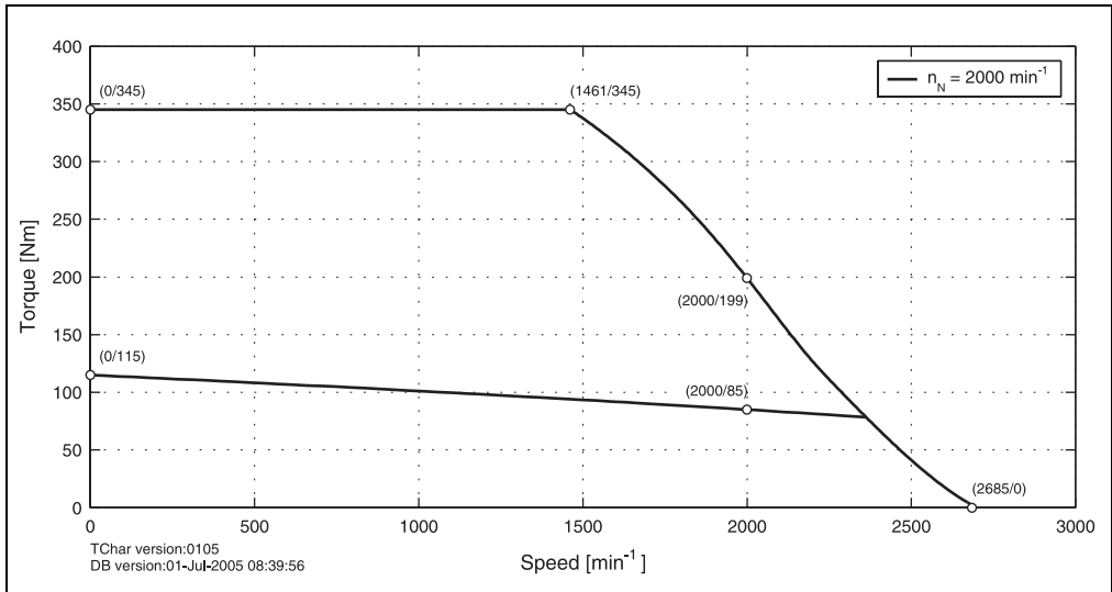
Figure 58: Speed - torque characteristic curve for 8LSA86.eennffgg-0
