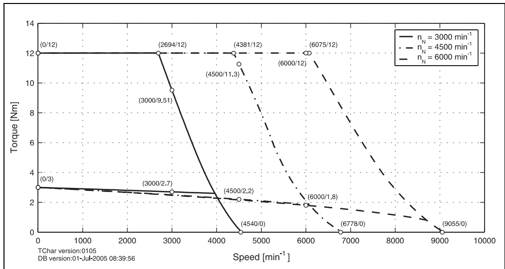
Figure 18: Speed - torque characteristic curve for 8LSA36.eennnffgg-0
