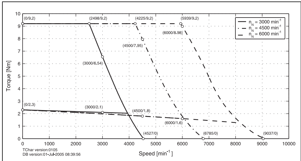
Figure 17: Speed - torque characteristic curve for 8LSA35.eennnffgg-0
