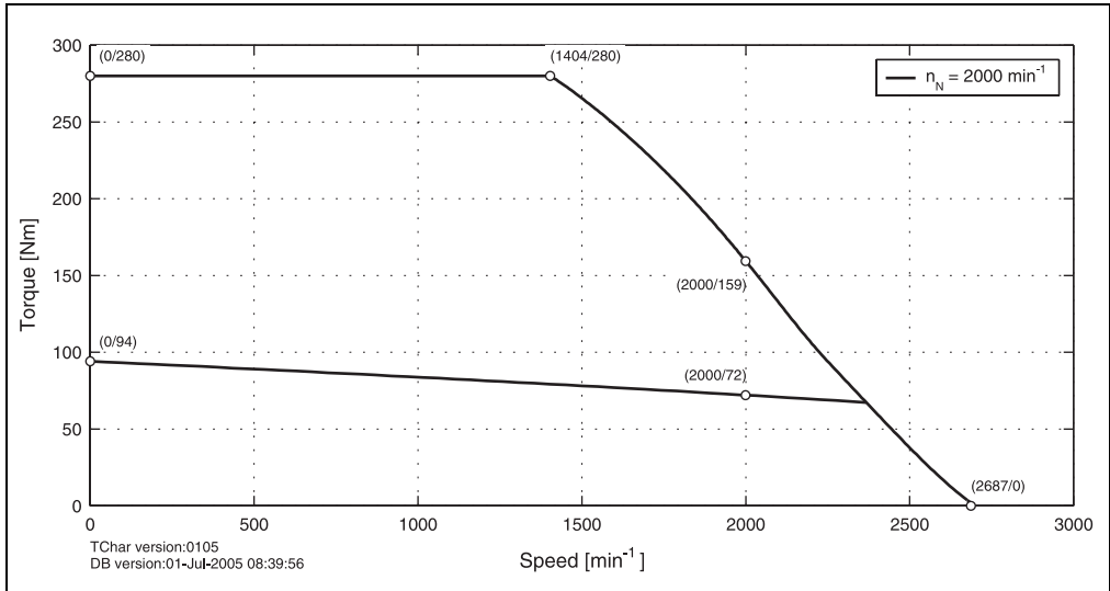
Figure 57: Speed - torque characteristic curve for 8LSA85.eennffgg-0
