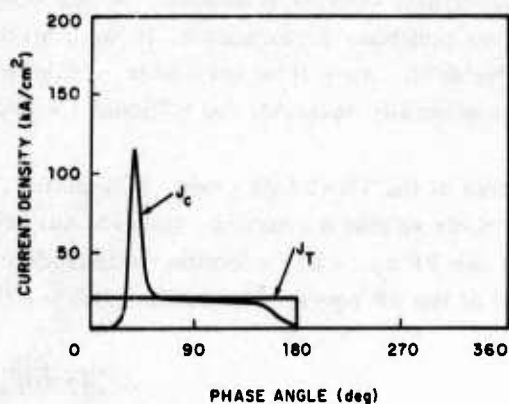
Fig. II-2. TRAPATT diode terminal waveforms.
