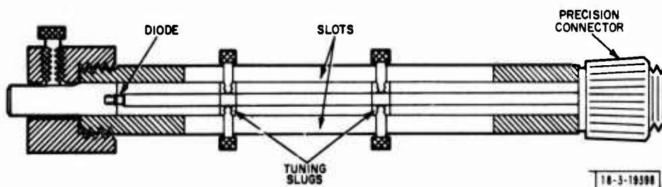
Fig. VI-25. Evans-type coaxial TRAPATT circuit.
