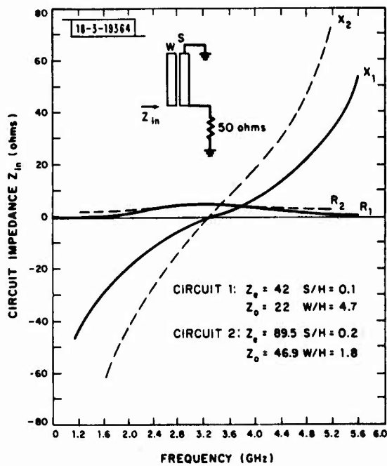
Fig. V-9. Impedance behavior of coupled-line transformers.
