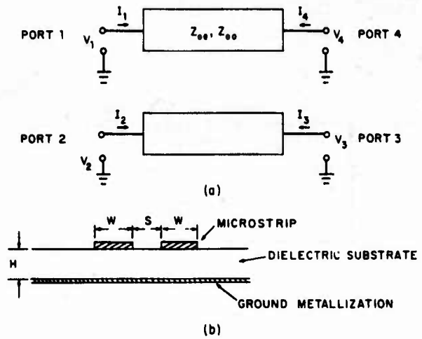
Fig. V-6. Coupled-microstrip transformer: (a) four-port coupled-line circuit and (b) side view of coupled-microstrip circuit.
