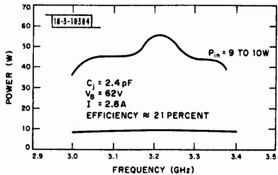
Fig. VI-10. Passband of Sperry 50-W amplifier.
