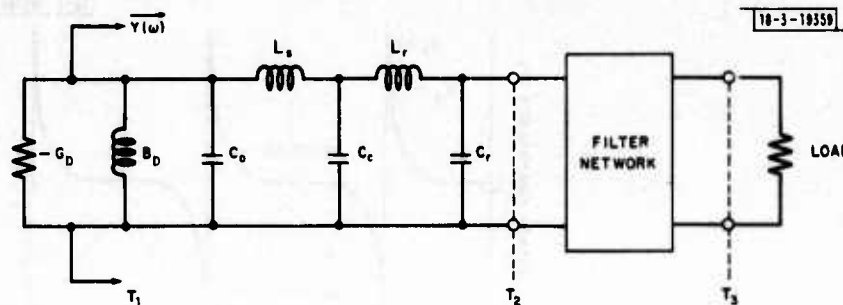
Fig. V-4. Large-signal equivalent circuit for wideband TRAPATT amplifier.
