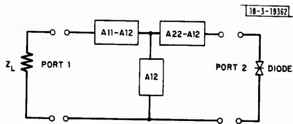
Fig. V-7. Two-port equivalent of coupled-microstrip circuit.
