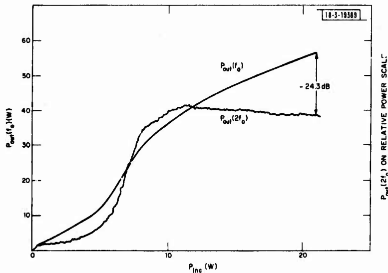
Fig. VI-16. Fundamental and 2nd harmonic vs incident power for 50-W S-band TRAPATT amplifier. V_B = 60 V; I_B = 3 A; attenuation = 20 dB; VSWR = 1.02; f_0 = 3.2 GHz; pulse length = 1 \mu sec; prf = 1 kHz; and duty factor = 0.1 percent. Assembly using two 3-port circulators.
