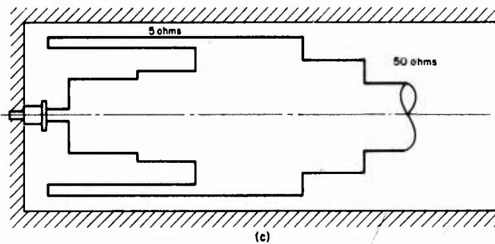
Fig. VI-27. Synthesis of distributed TRAPATT load: (a) lumped element, (b) alternate configuration, and (c) coaxial realization.
