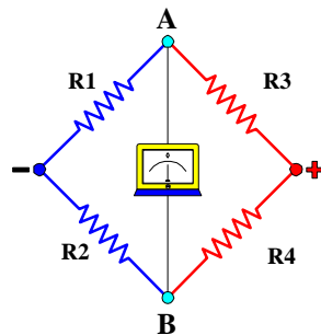
Basic Wheatstone Bridge
