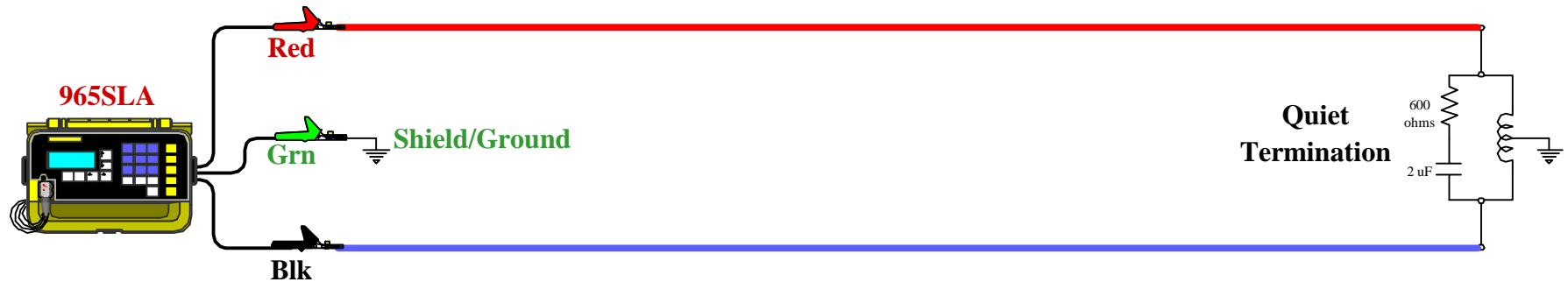
Fig. 1: Circuit Noise (Noise Metallic) is measured between Tip[A] & Ring[B]
