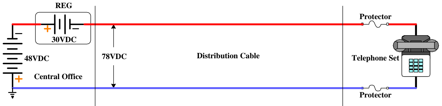
Fig. 2: Telephone Circuit with REG (Range Extender with Gain).
