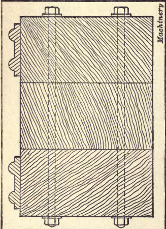
Fig. 2. Built-up Wooden Lathe Bed provided with Iron Ways
