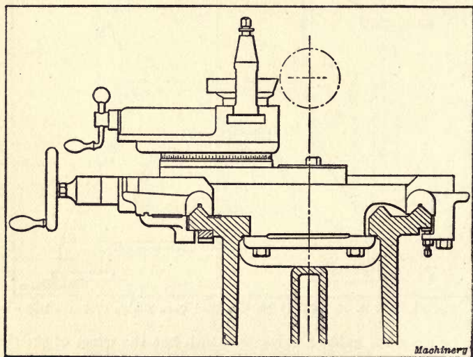
Fig. 35. The Lodge & Shipley Machine Tool Co.'s Lathe Bed with Supplementary Bearing Surface
