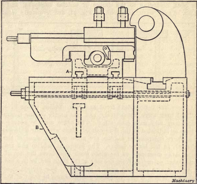
Fig. 60. The Dron & Lawson, Ltd., Glasgow, Scotland, Lathe with Extensions carrying Supplementary Bed for Carriage
