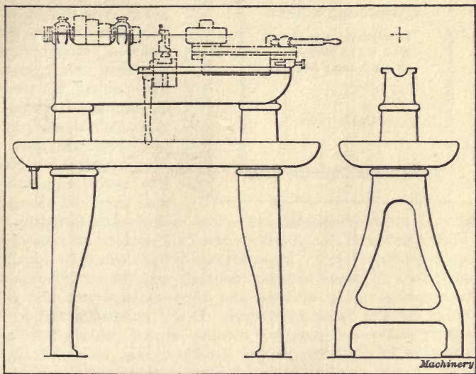
Fig. 73. Turret Lathe Bed with Head cast Solid with it
