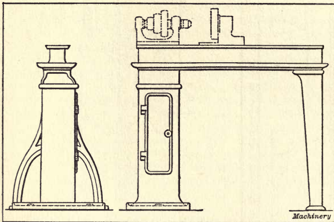
Fig. 64. Bed for Small Lathe
