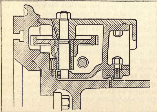
Fig. 49. Support for Apron on a Heavy Lodge & Shipley Lathe
