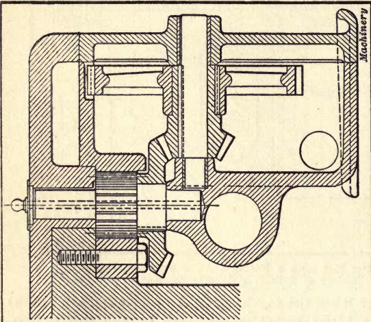
Fig. 50. Vertical Rack and Pinion on Lathe built by Joshua Buckton & Co., Ltd., Leeds, England
