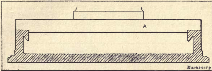
Fig. 11. Early Type of Bed for Heavy Lathes
