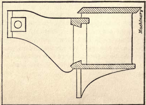
Fig. 4. Early Front Slide Lathe Bed
