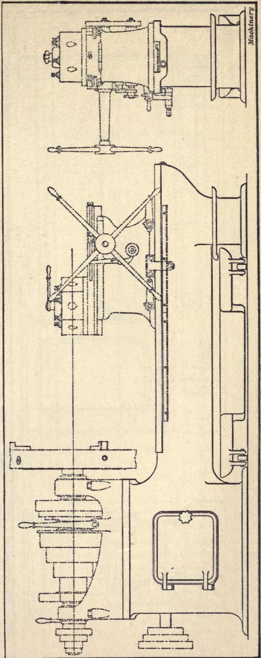
Fig. 66. Type of Bed used for Chucking Lathe
