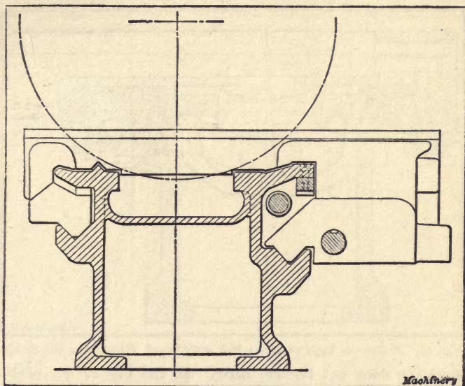
Fig. 52. Bed with Lower-tier Vee-ways as designed by Schaerer & Co., Karlsruhe, Germany
