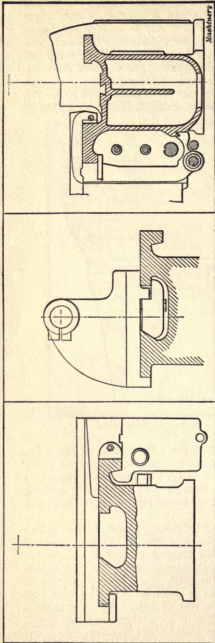
Fig. 45. Lathe Bed with Inverted Narrow Guide, designed by Ward, Haggas & Smith, Keighley, England
