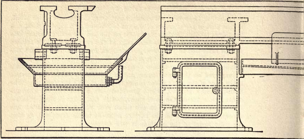
Fig. 37. Lathe Bed supported on Cabinet Standards
