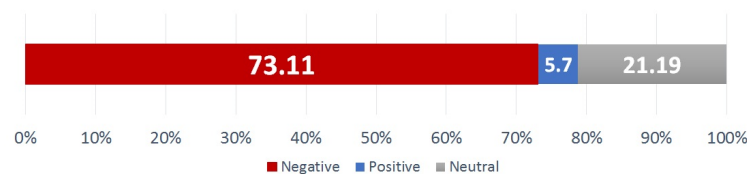
Fig. 4: Sentiment Orientation
