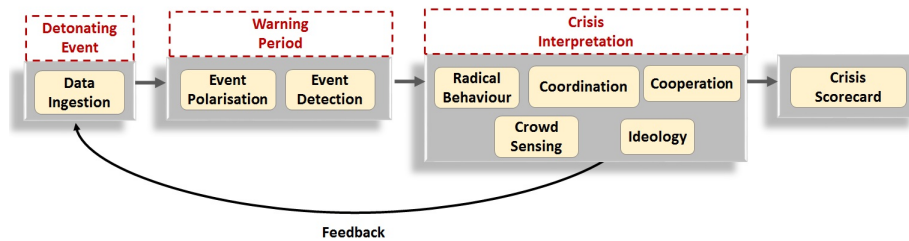
Fig. 2: Conceptual Model
