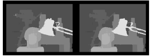
Figure 5. Disparity map of the left Tsukuba image before (left) and after (right) occlusions and mismatches have been handled.
