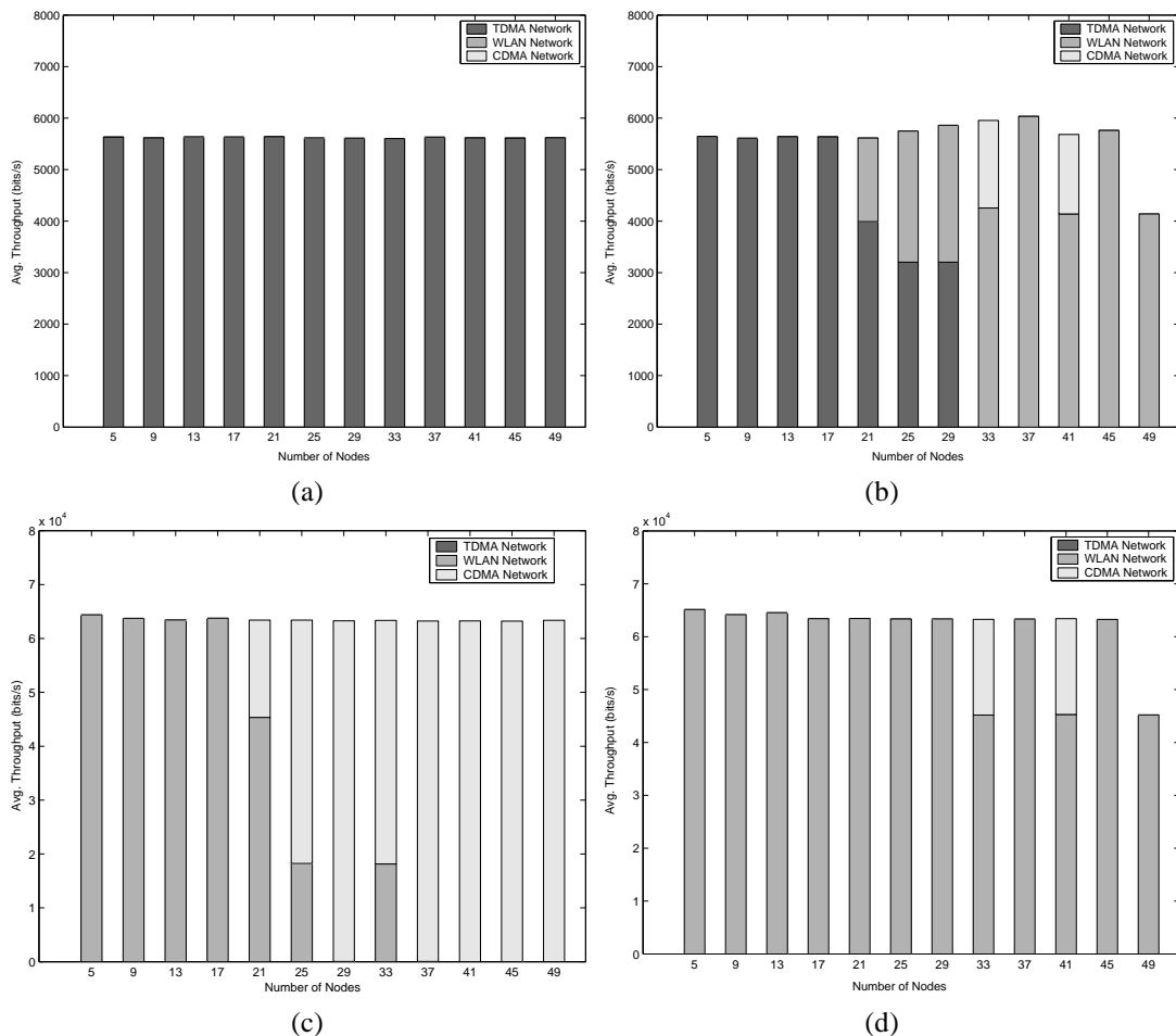
Fig. 5. Average throughput of voice traffic with (n_T, n_C, n_W) = (a)(10%, 10%, 80%), (b)(50%, 30%, 20%), and CBR traffic with (n_T, n_C, n_W) = (c)(10%, 10%, 80%), (d)(50%, 30%, 20%).
