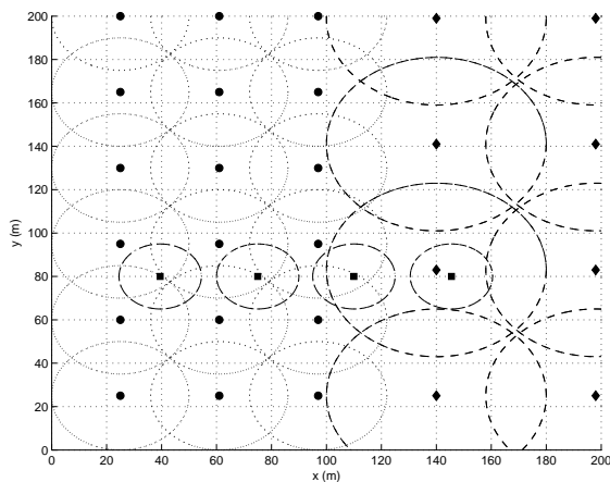
Fig. 7. Sample topology used in the mobility simulations. \bullet : TDMA BS, \blacklozenge : CDMA BS, \blacksquare : WLAN AP.
