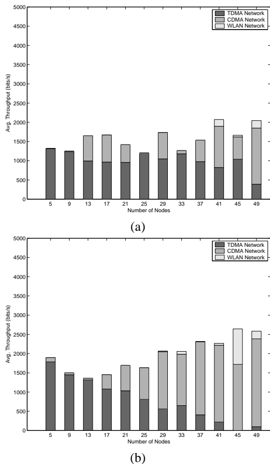
Fig. 6. Average throughput of best-effort traffic with (n_T, n_C, n_W) = (a)(10%, 10%, 80%), (b)(50%, 30%, 20%).
