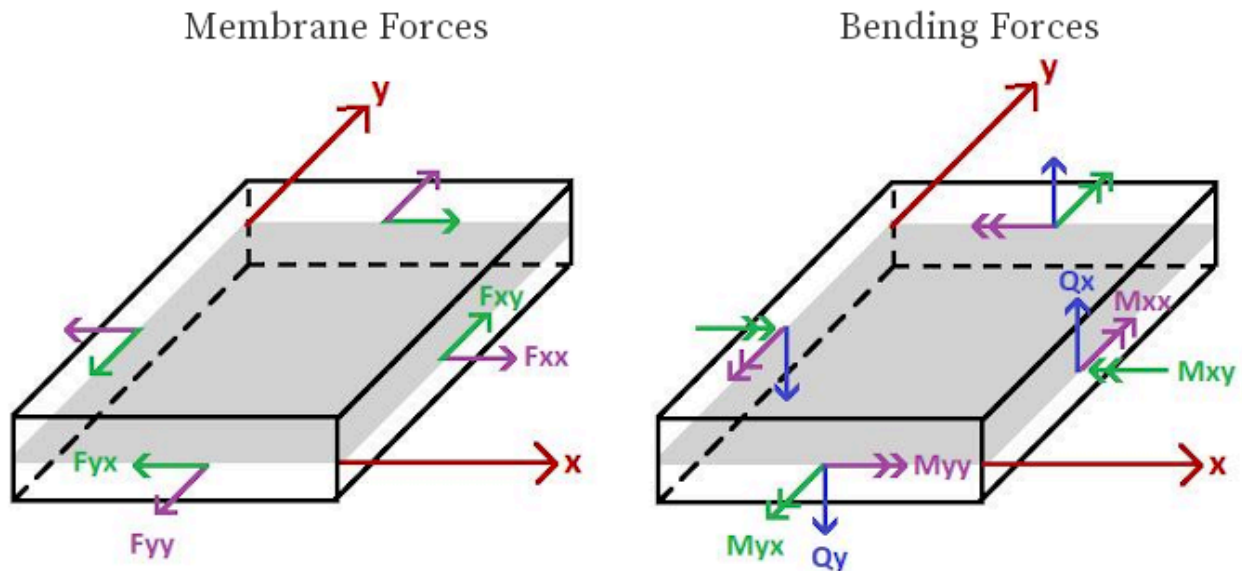
Plate Internal Force Directions
