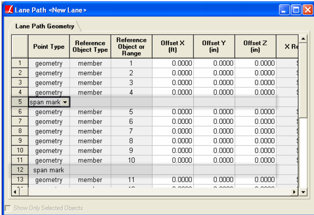
Span Break Markers in the Lane Path Definition
