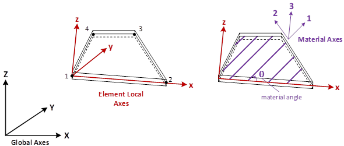
Plate Local Axes (left) and Material Axes (right)
