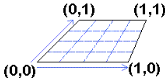
Load coordinate specification for quadrilateral plates
