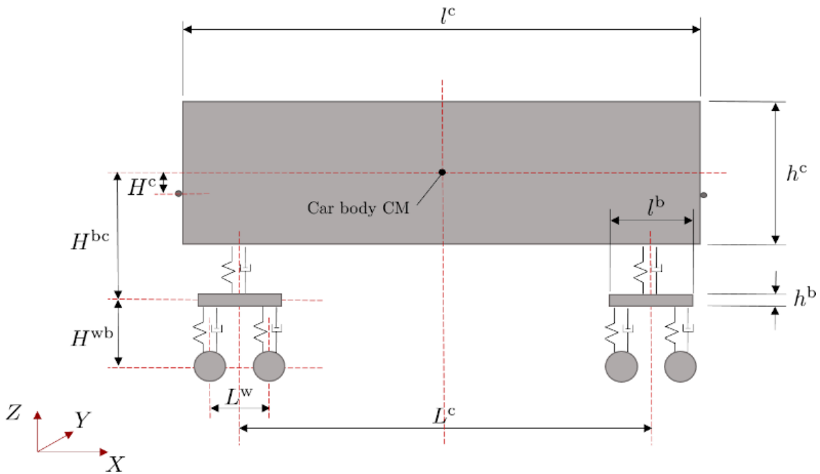
Geometric properties of a VTSI Parametric Car
