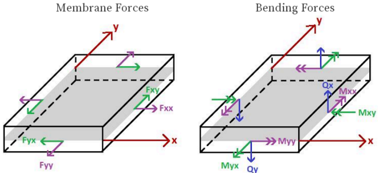
Plate Internal Force Directions
