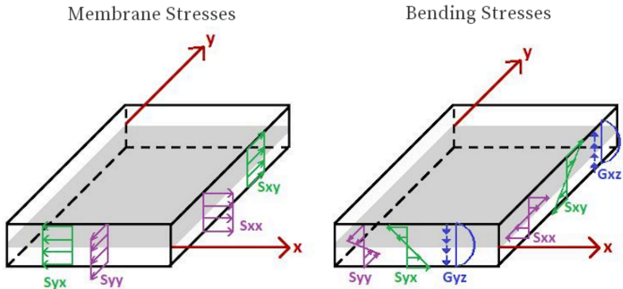
Plate Stress Directions
