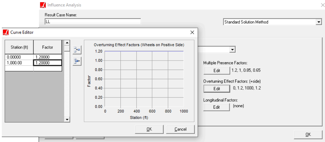
Overturning Effect Factors
