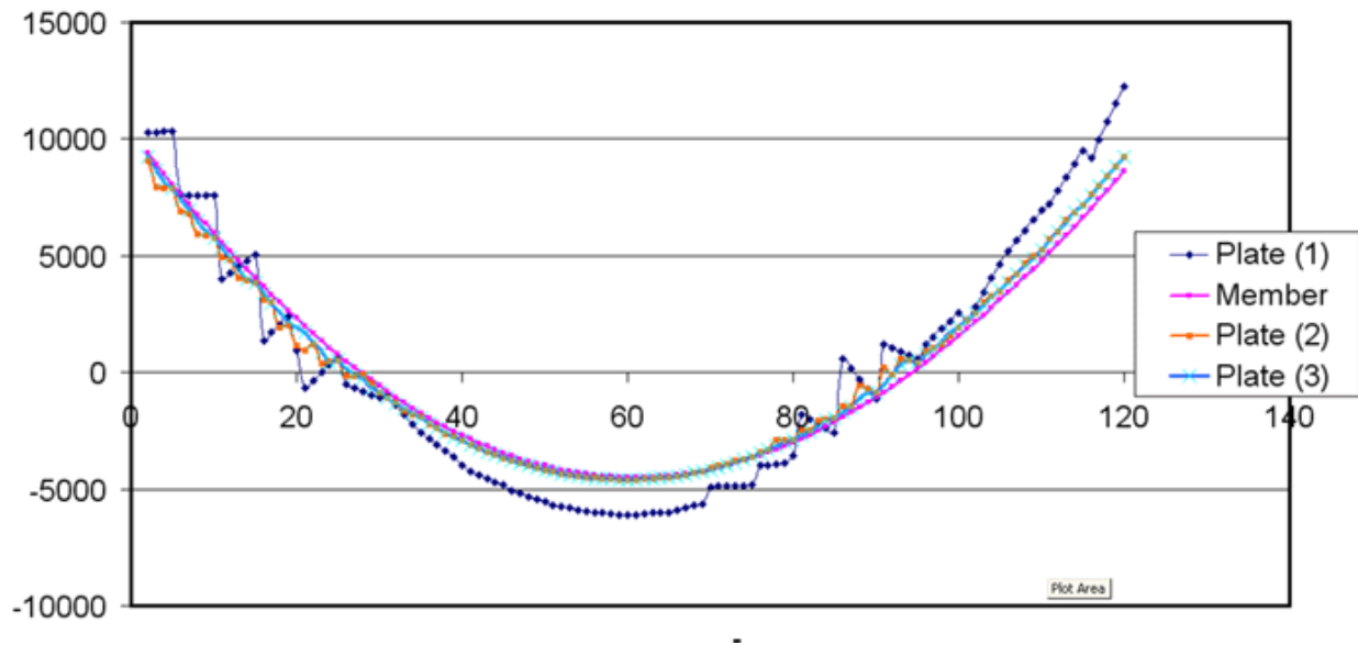
Figure 4: Comparison of Compound Element Forces and Member Sectional Forces for an Equivalent Model, for different plate mesh sizes
