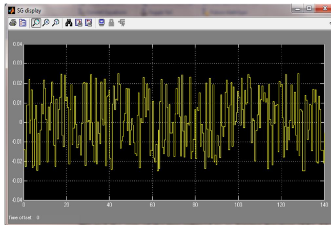
Figure 4.6: Signal generator; generates random periodic forces, amplitude = 0.025, frequency = 1.0 rad/sec
