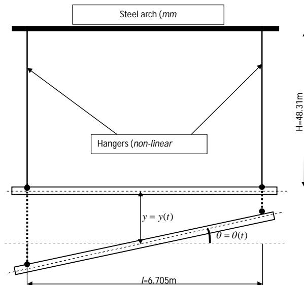
Figure 4.1: Mathematical model of cross section of Adomi Bridge
