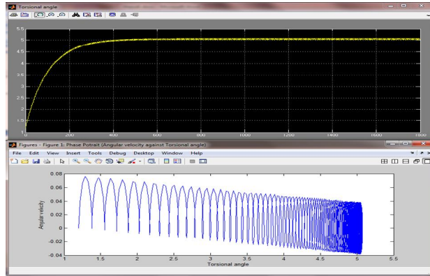
Figure 4.5. Torsional motion; Bridge response for K=0 , f(t)=0.05\sin 1.3t and Phase portrait
