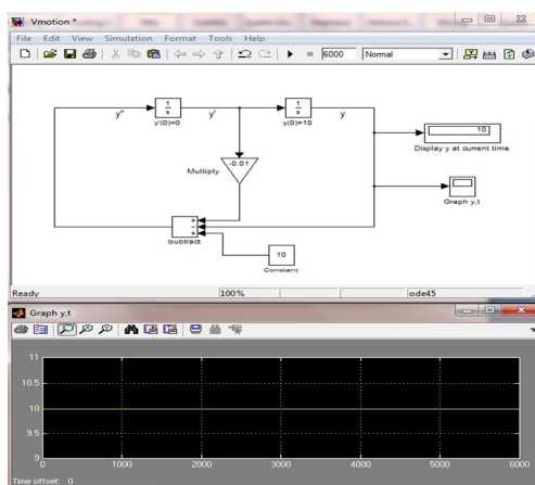
Figure 4.3: SIMULINK Scheme for vertical motion and the bridge response y(0) = 10
