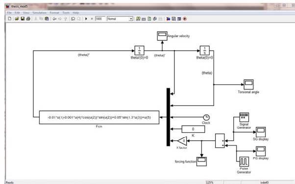
Figure 4.4: SIMULINK Scheme for torsional motion of bridge deck
