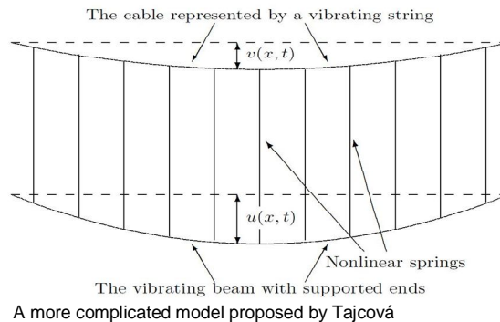
A more complicated model proposed by Tajcová
