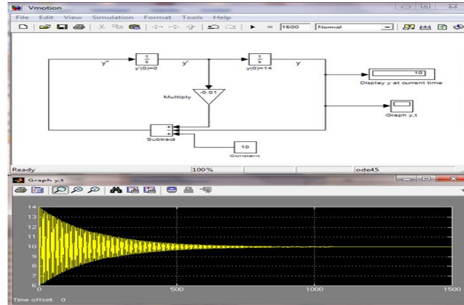
Figure 4.2: SIMULINK Scheme for vertical motion and the bridge response, y(0) = 14
