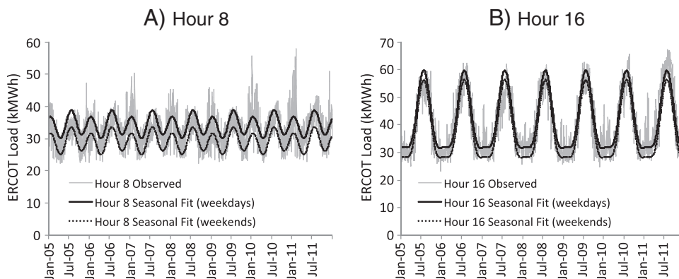
Fig. 2. ERCOT load over 2005–11 for chosen hours, along with fitted seasonality functions.
