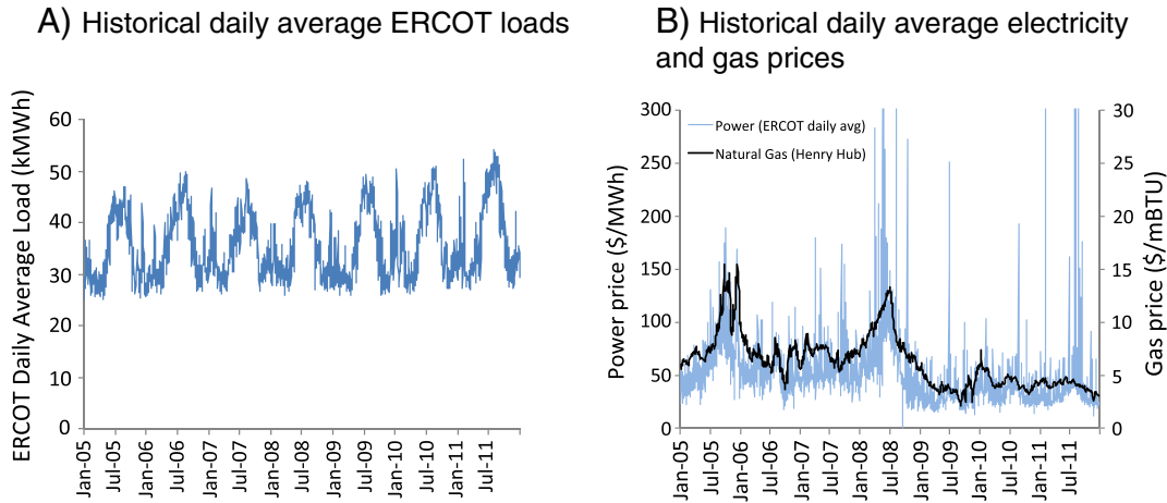
Fig. 1. ERCOT load and electricity prices over 2005–11. Note that we choose to plot daily average power prices only for the range $0 to $300. However, during the period 2005–11, there were nine days with averages above $300 (including five in August 2011), and two days in Sept 2008 with averages just below zero (due to several hourly values below –$200).
