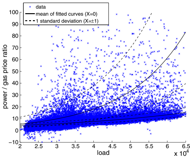
Fig. 4. Fitting result – solid lines illustrate exponential price–load relationship when X = 0 (at the mean), while dotted lines represent one standard deviation bands ( X = \pm 1 ). The y-axis has been truncated for illustration purposes: min and max values are -38 and 450 respectively.
