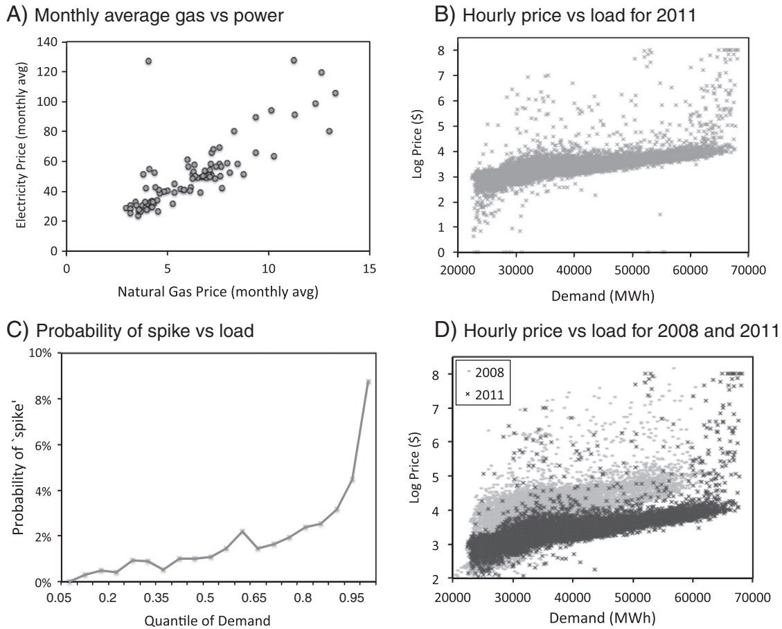
Fig. 3. Relationship between power price and gas price (top left), between power price and load (right column), and between spike probability and load (bottom left).
