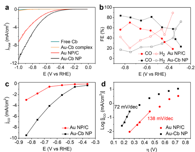
Figure 4. (a) LSV scans of Au–Cb NP, Au NP/C, free carbene and molecular Au–Cb complex under \text{CO}_2 -saturated 0.1 M \text{KHCO}_3 at pH 6.8. (b) Faradaic efficiencies of products formed from Au–Cb NP and Au NP/C. (c) Specific CO current density (based on electrochemically active surface area) plots for Au–Cb NP and Au NP/C. (d) Tafel plots of Au–Cb NP and Au NP/C.
